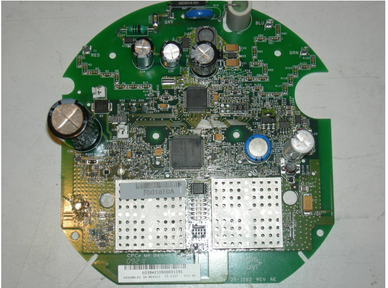
Figure 2: PCB with Shields - Front
