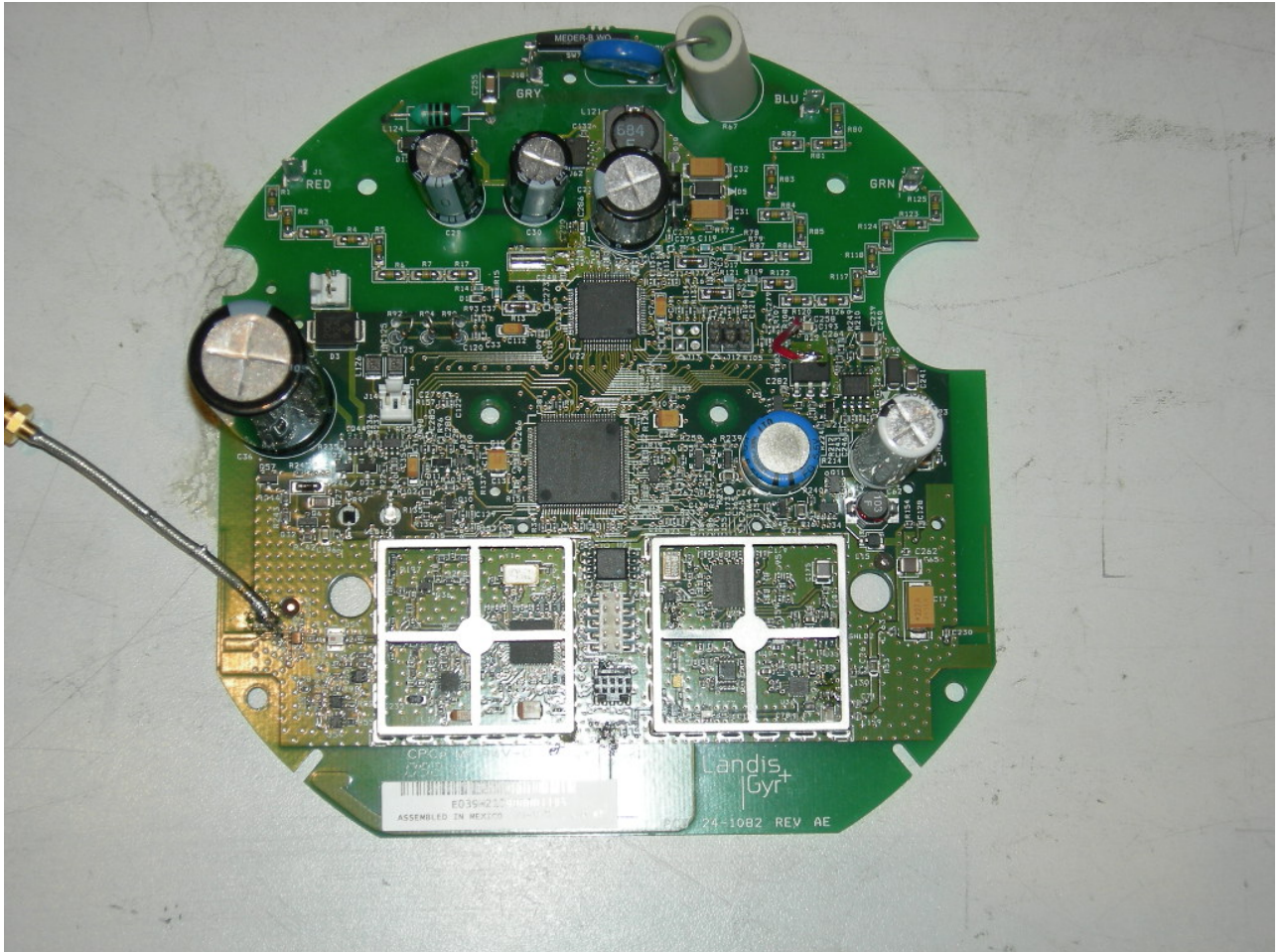
Figure 3: PCB without Shields - Front
