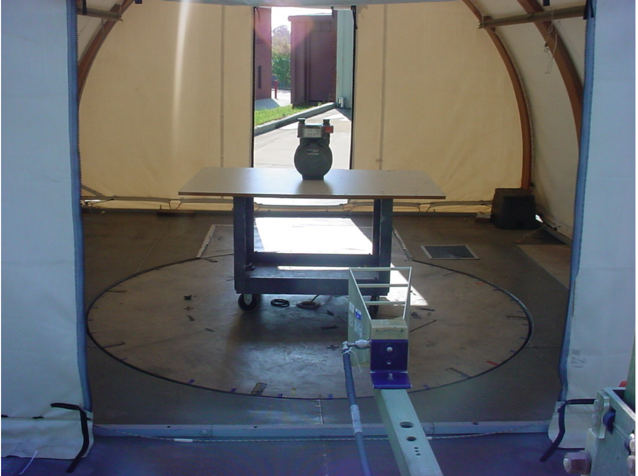
Figure 3: 25-1080 – Radiated Emissions
