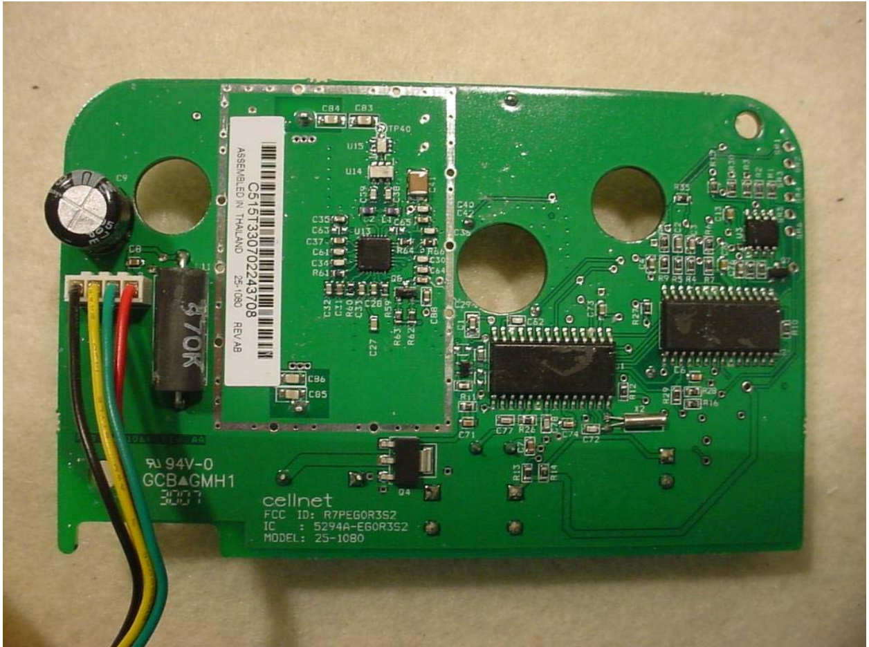
Figure 3: 25-1080 PCB– Front
