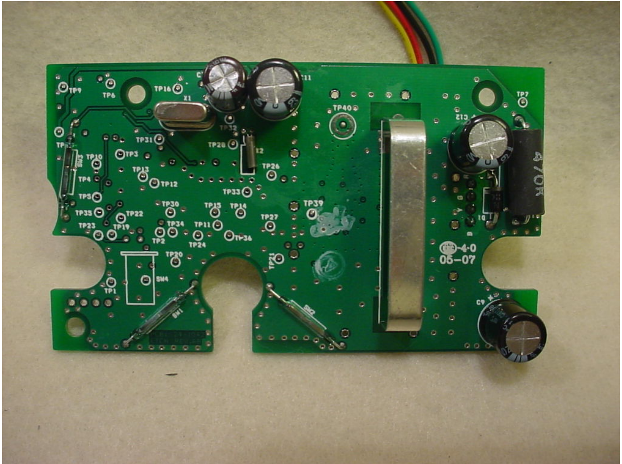
Figure 2: 25-1075 PCB - Back
