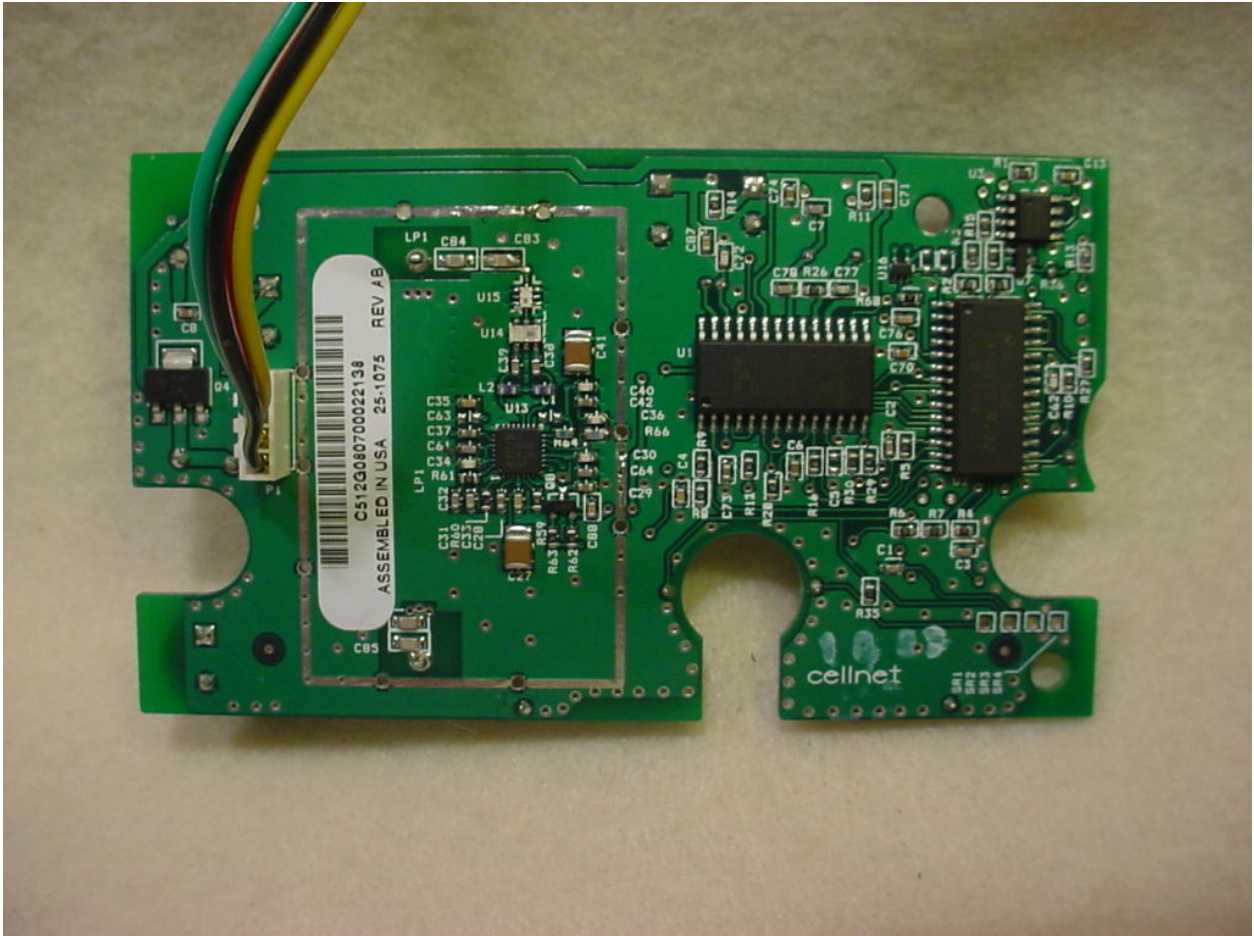
Figure 1: 25-1075 PCB – Front
