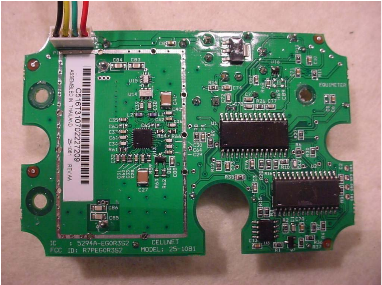
Figure 5: 25-1081 PCB – Front
