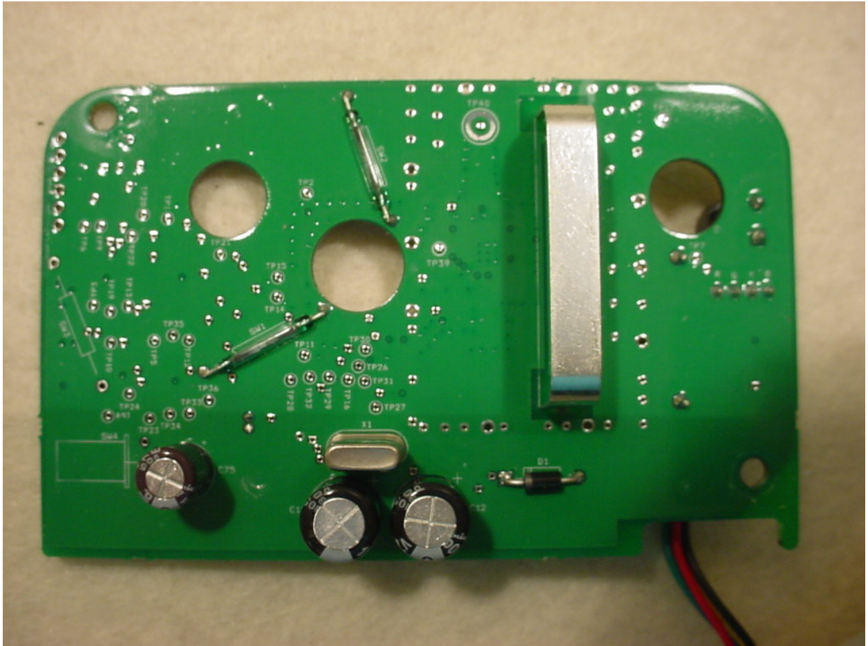
Figure 4: 25-1080 PCB - Back
