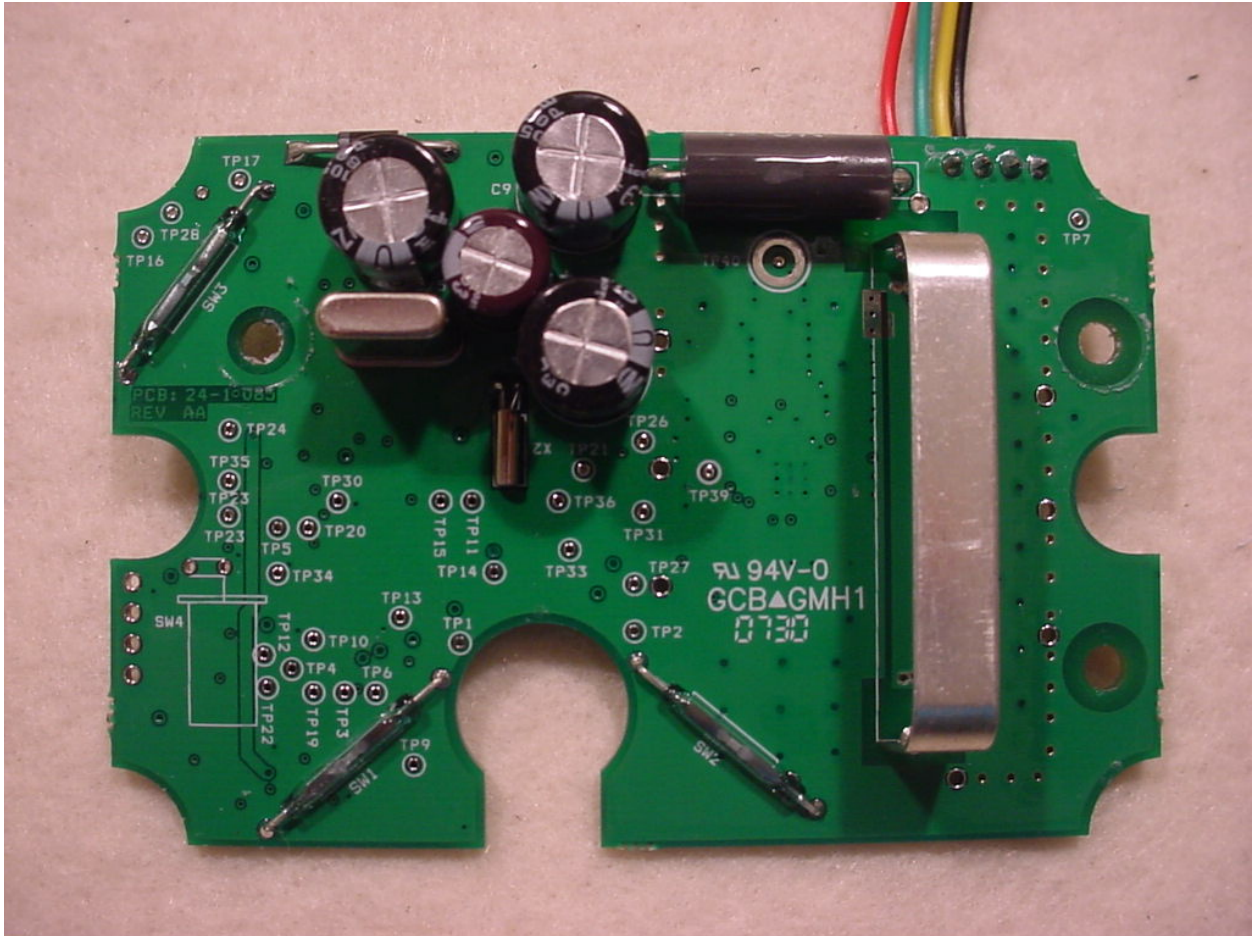
Figure 6: 25-1081 PCB - Back
