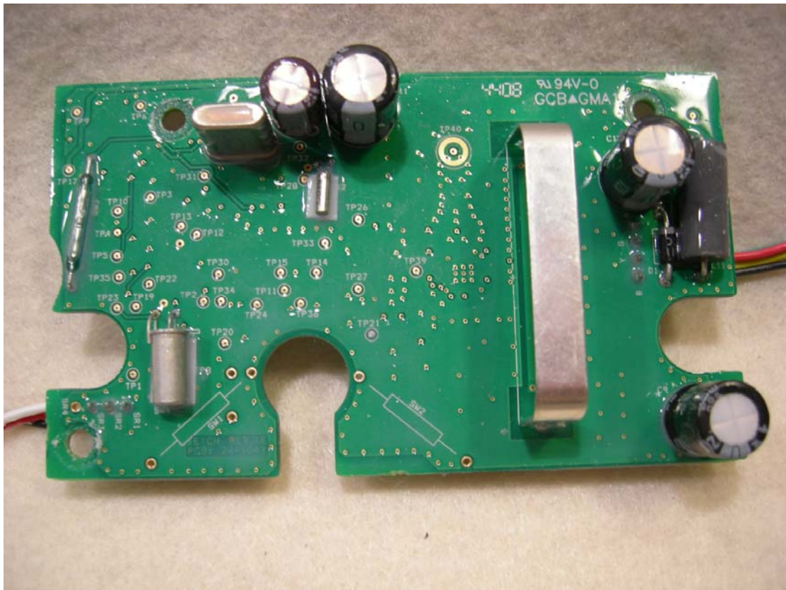
Figure 2: PCB - Back
