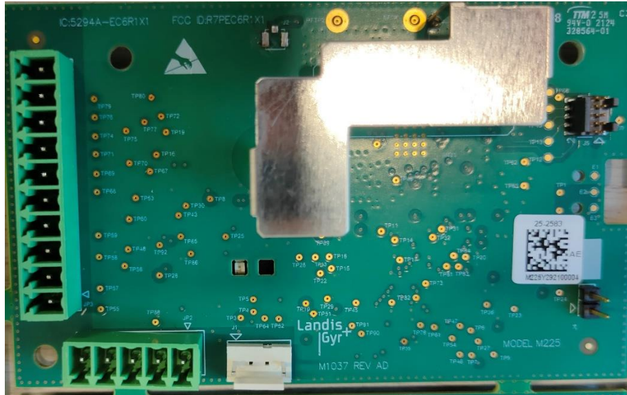
Figure 3. Top side with Antenna
