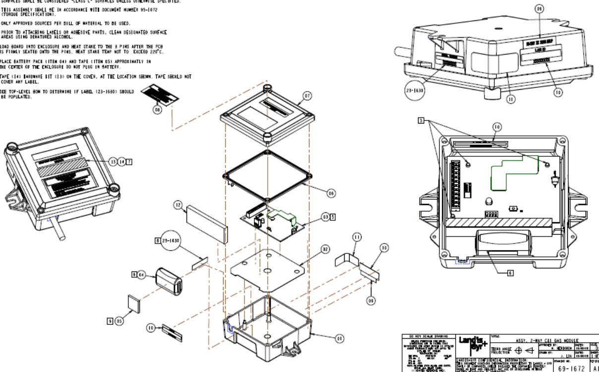
Figure 4. Products Containing the M225 PCBA
