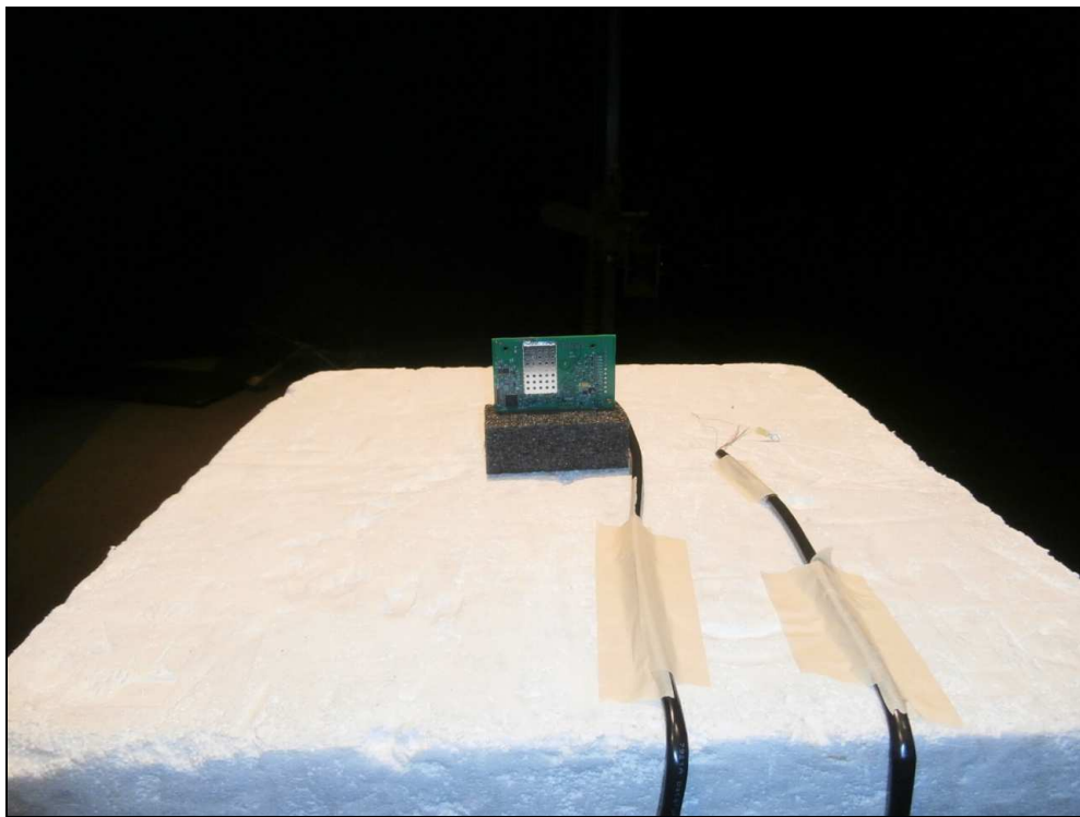
Figure 4: Radiated Emissions
