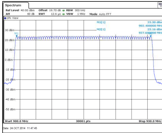
Figure 7.4.2.2-11: Mode 4 (64 Channels)
