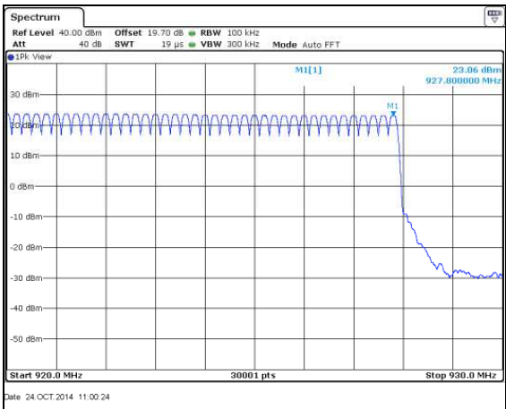
Figure 7.4.2.2-10: Mode 3 (129 Channels)
