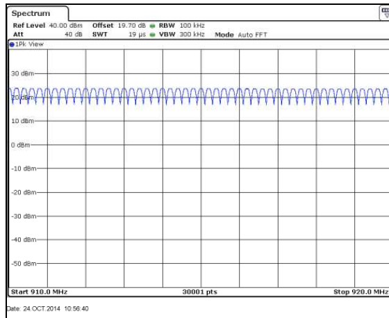
Figure 7.4.2.2-9: Mode 3 (129 Channels)
