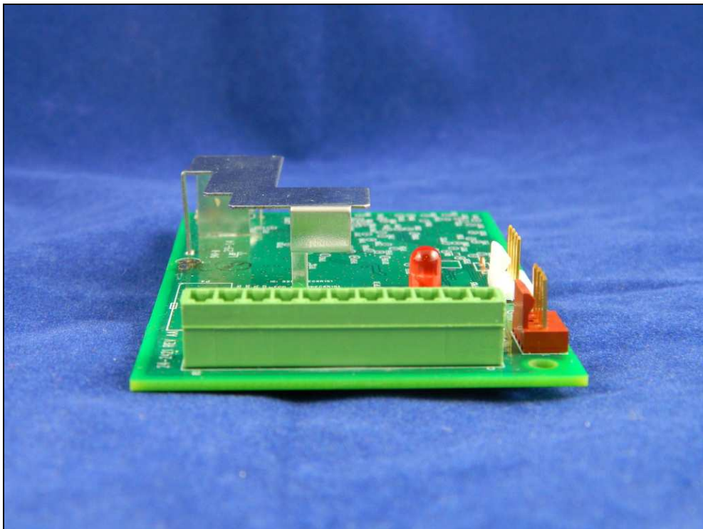
Figure 6: External Photo
