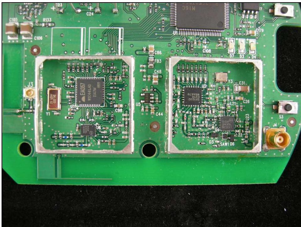
Figure 2: Internal Photo – Shields Removed (Close-up)
