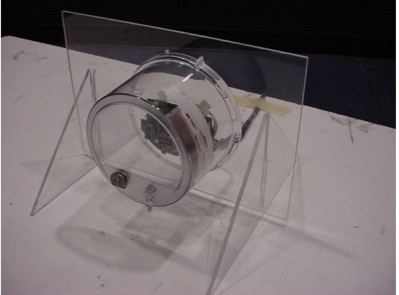
Figure 1: Test Setup - Radiated Emissions – Intentional
