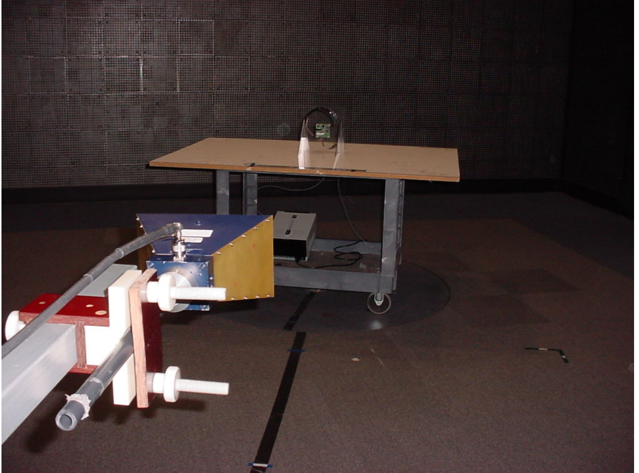
Figure 2: Test Setup - Radiated Emissions – Intentional
