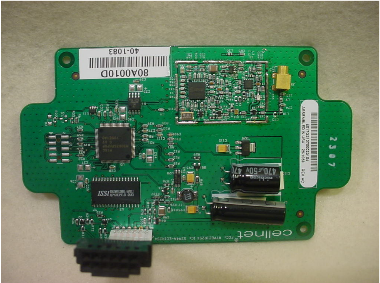
Figure 2: Internal Photographs – PCB Front (No Shield)
