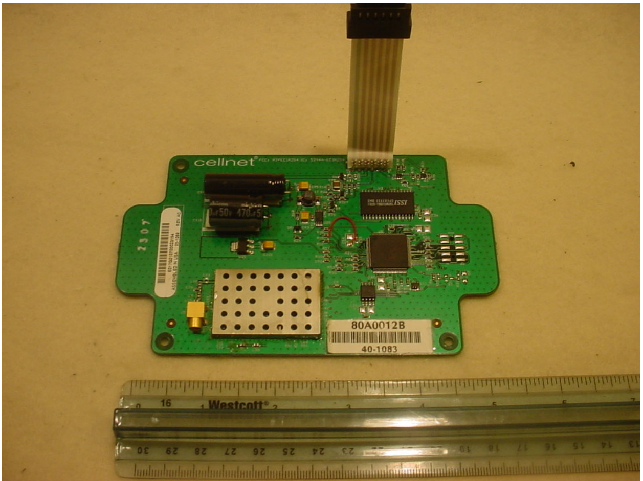
Figure 1: Internal Photographs – PCB Front
