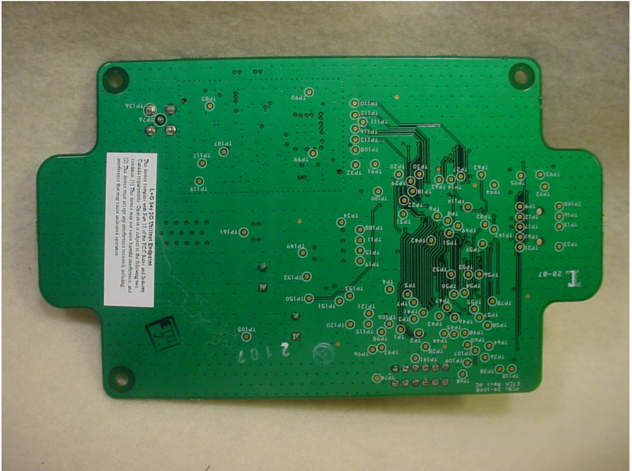
Figure 3: Internal Photographs – PCB Back
