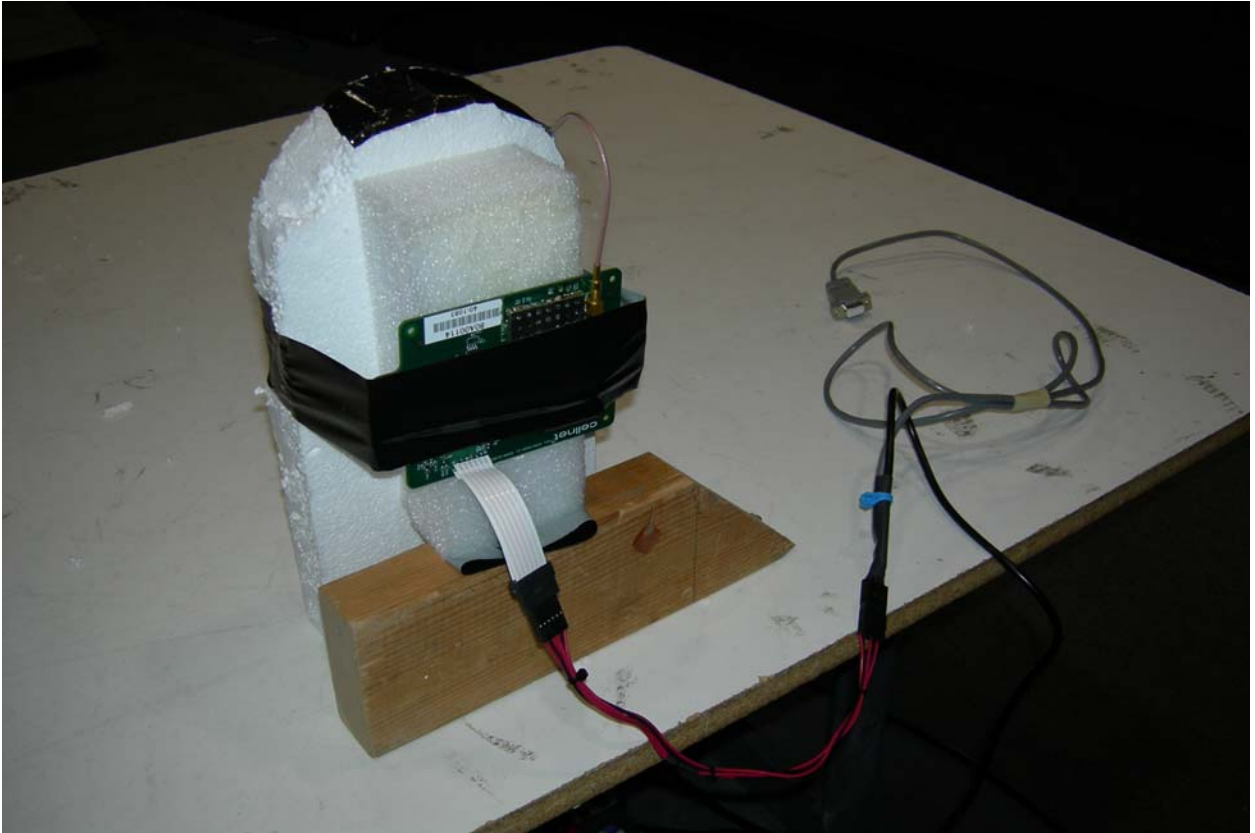
Figure 3: Test Setup - Radiated Emissions – Unintentional
