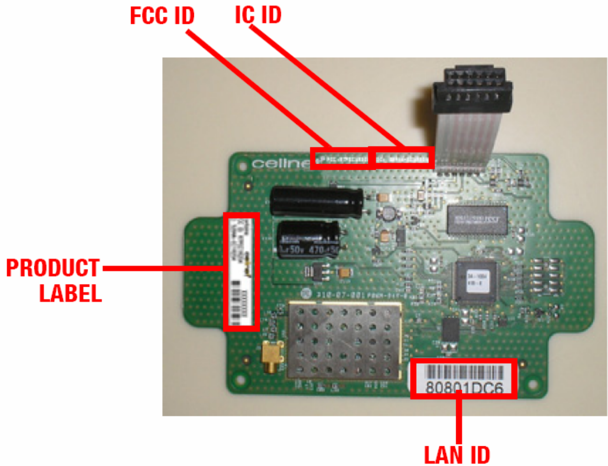
Figure 1: Label Location – PCB Front
