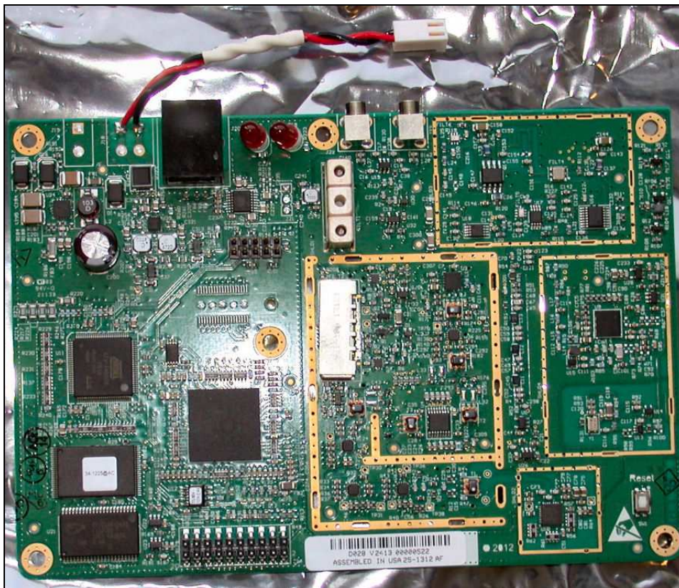
Figure 2: Internal Photo – BLT5 Top without Shields
