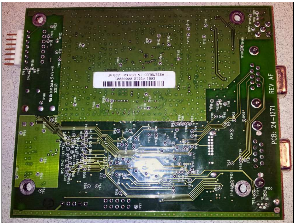
Figure 6: Internal Photo – IWR Bottom
