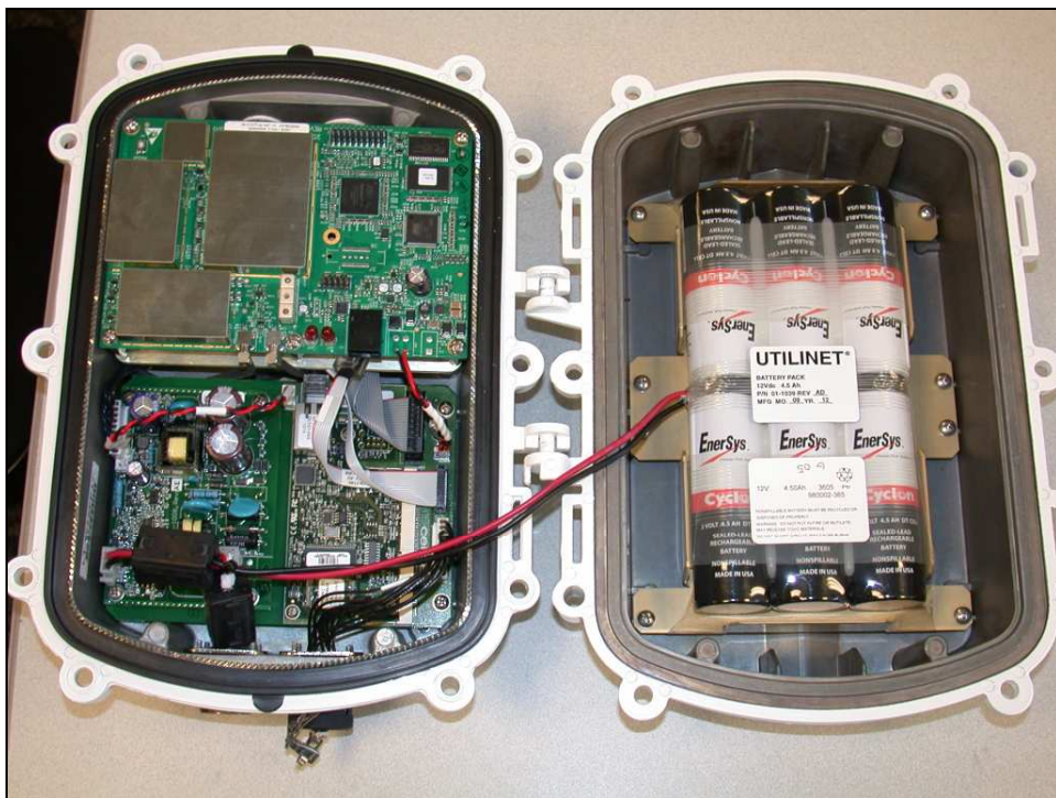
Figure 7: Internal Photo – Series-4 Concentrator Assembled with BLT5 and IWR
