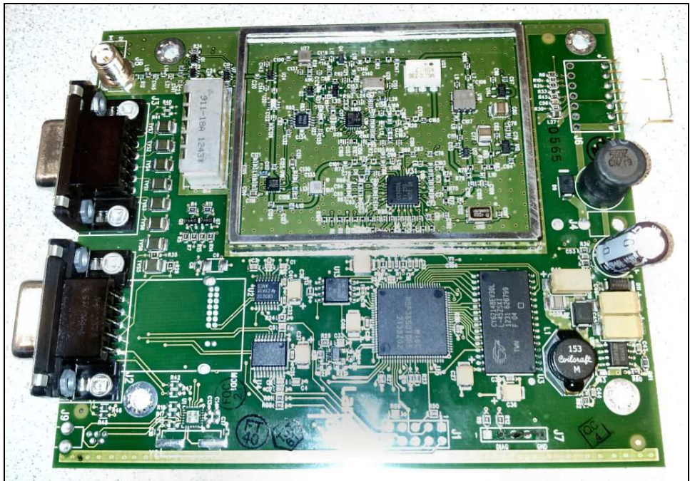
Figure 5: Internal Photo – IWR Top without Shields
