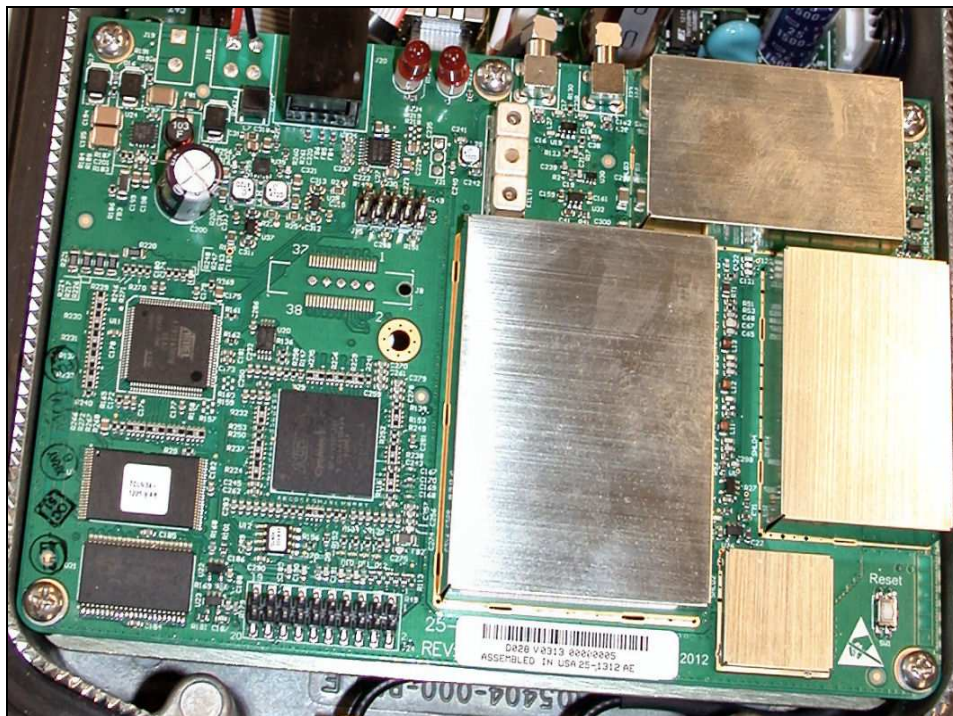
Figure 1: Internal Photo – BLT5 Top with Shields
