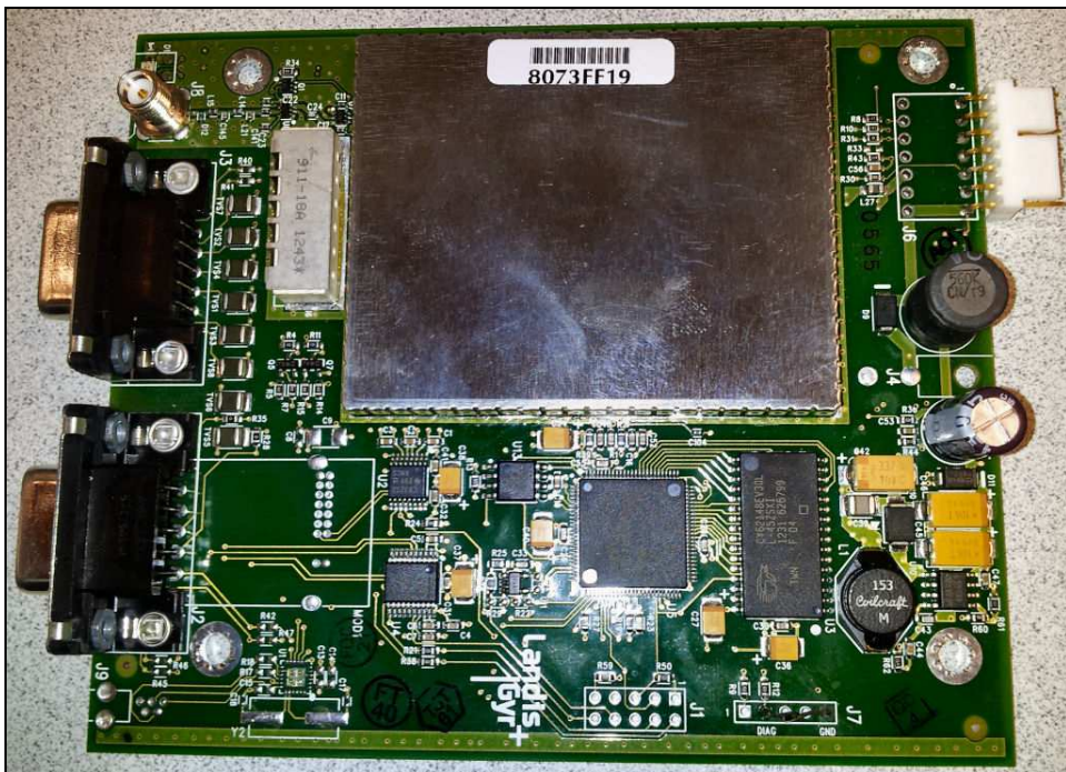
Figure 4: Internal Photo – IWR Top with Shields
