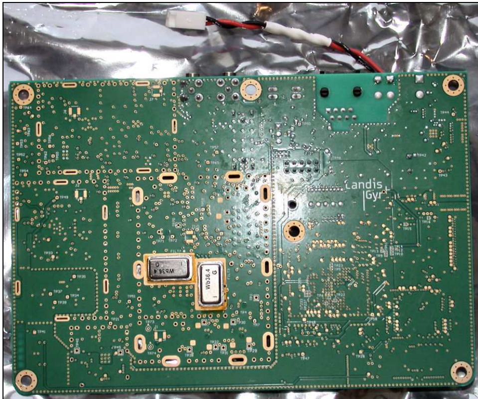
Figure 3: Internal Photo – BLT5 Bottom
