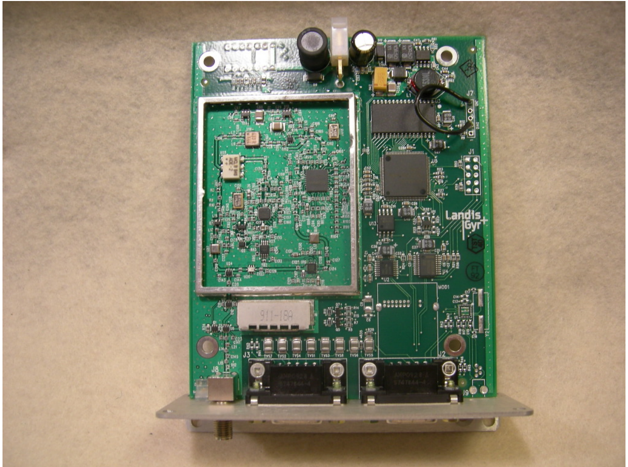
Figure 3: WAN (Utilinet IWR) PCB Front
