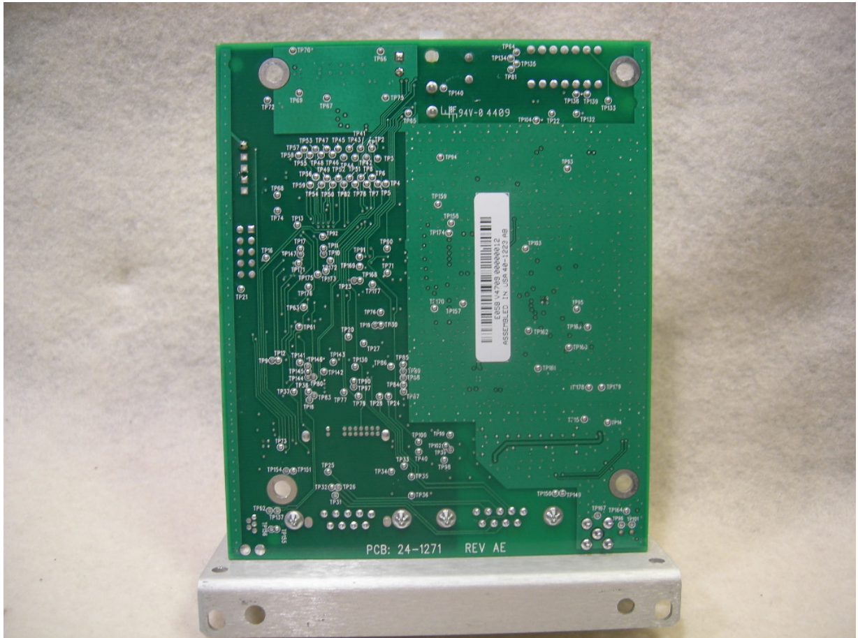
Figure 4: WAN (Utilinet IWR) PCB Back
