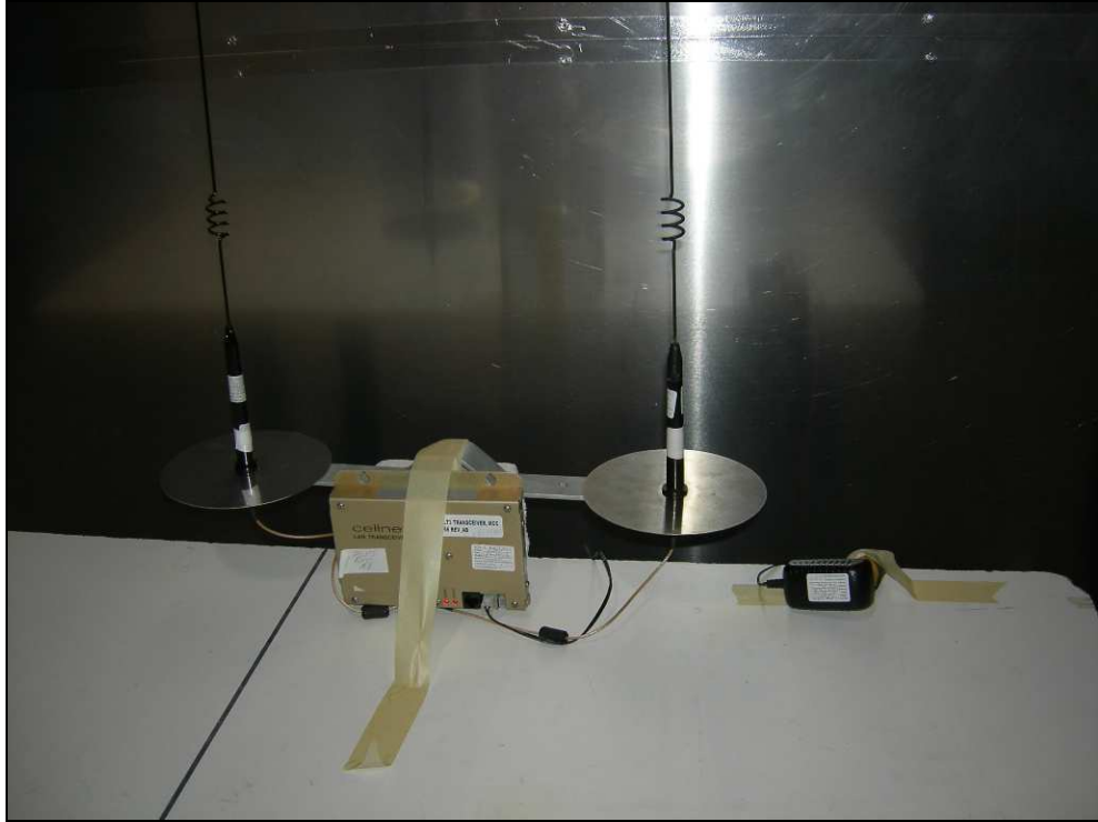
Figure 7: Conducted Emissions
