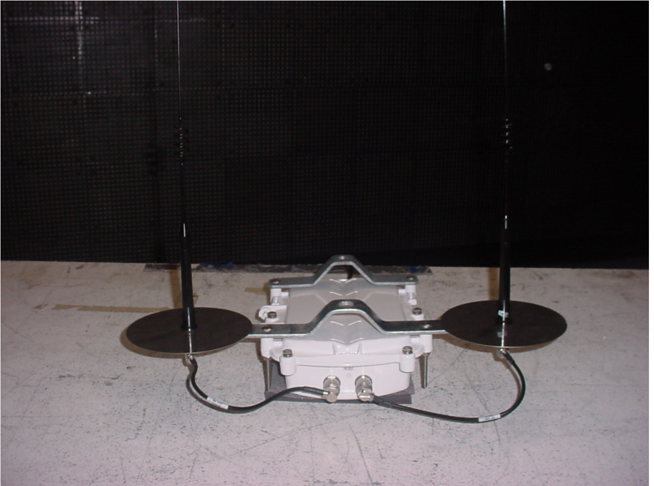
Figure 2: Test Setup – Radiated Emissions – Close Up
