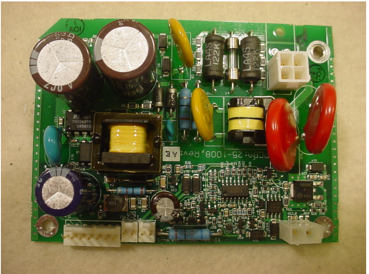
Figure 5: Power Supply Board - Top View
