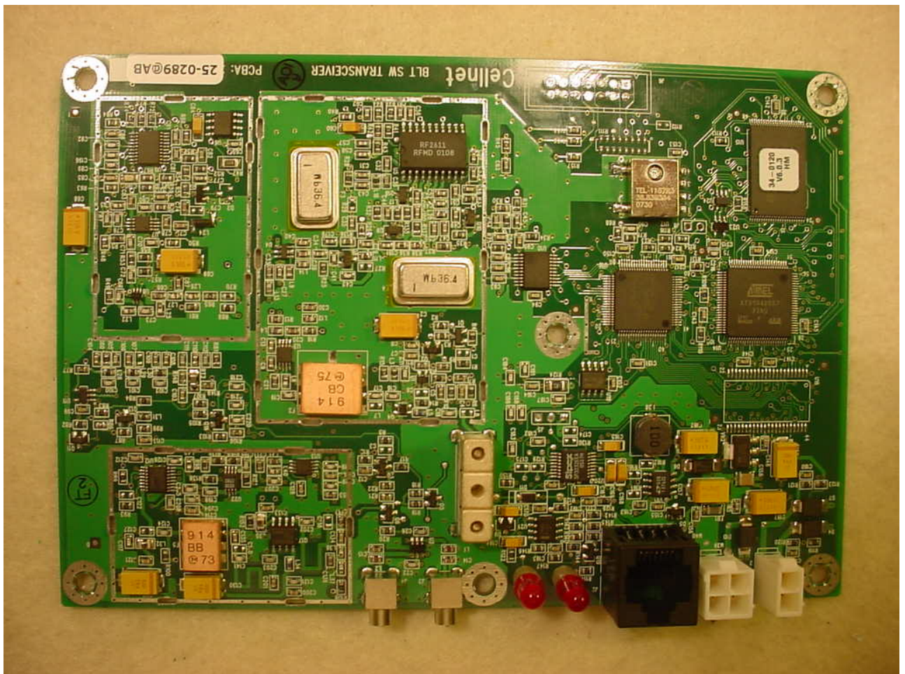
Figure 3: RF Board - Top View without Shields
