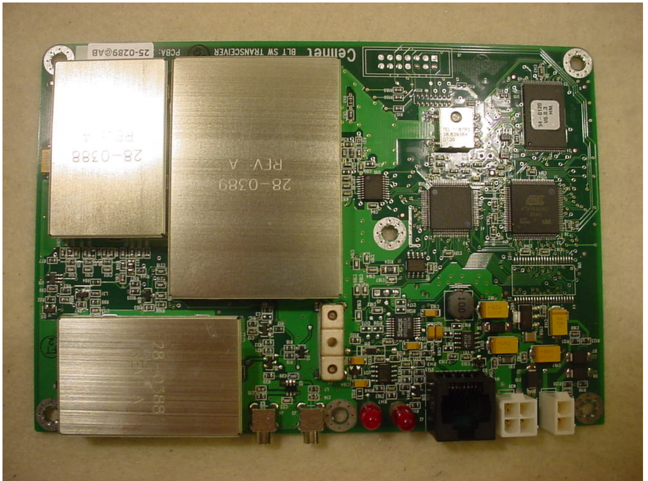
Figure 2: RF Board - Top View with Shields
