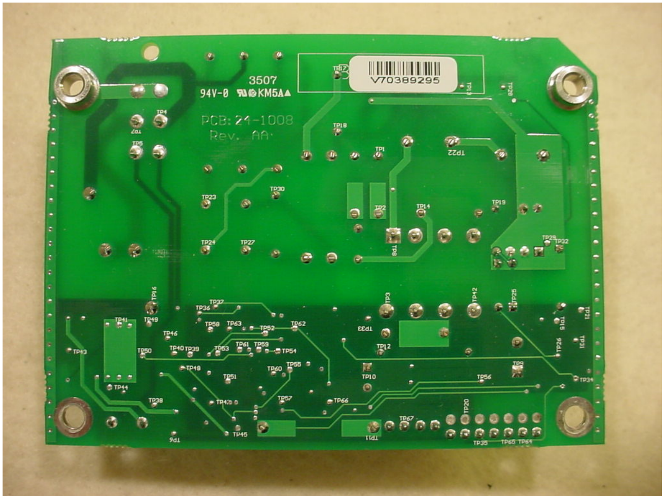
Figure 6: Power Supply Board - Bottom View
