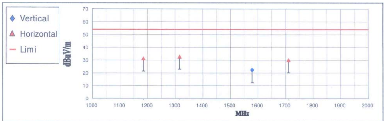
< Fig 7. Radiated Emission result _ Digital (1000MHz ~ 2000MHz) >
