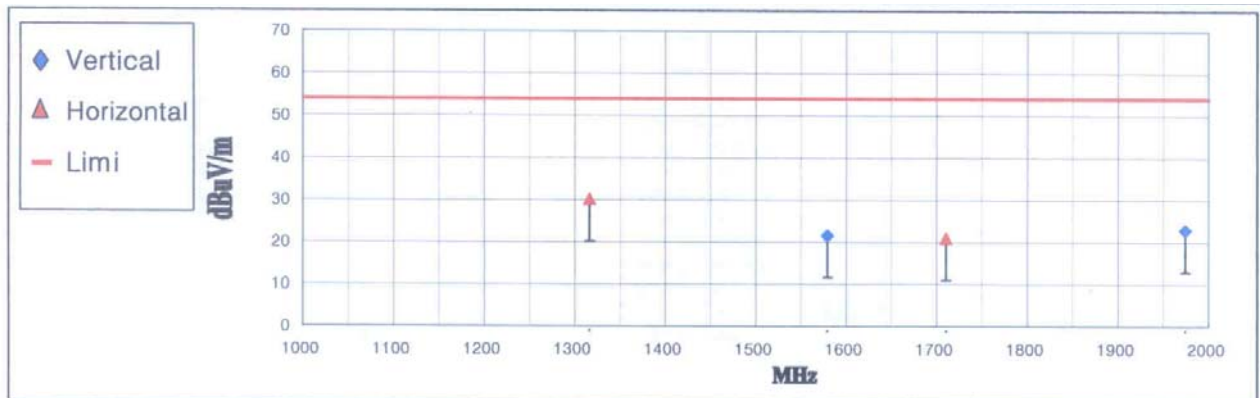
< Fig 5. Radiated Emission result _ Analog (1000MHz ~ 2000MHz) >
