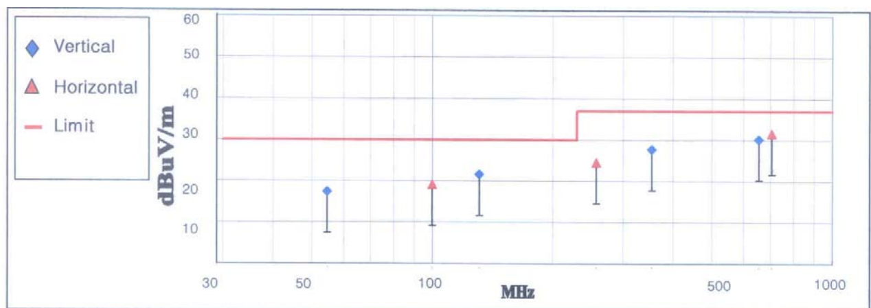
< Fig 4. Radiated emission result _ Analog (30MHz ~ 1000MHz)>
