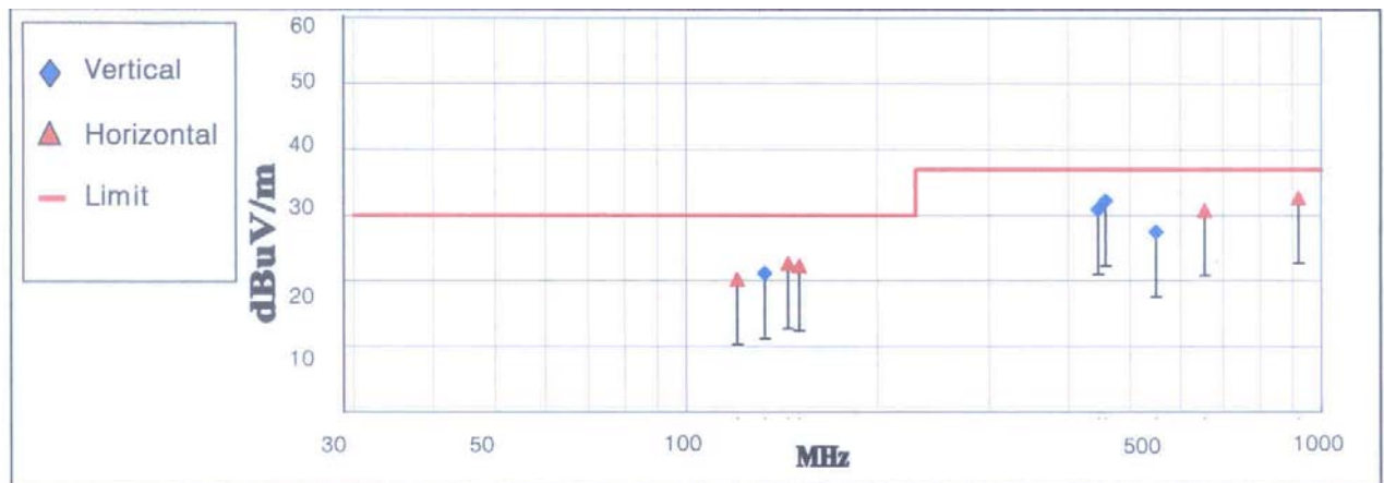
< Fig 6. Radiated emission result _ Digital (30MHz ~ 1000MHz)>
