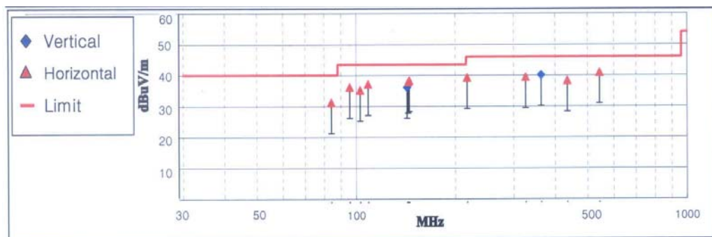
-. Fig 5. Radiated emission result _ Digital
