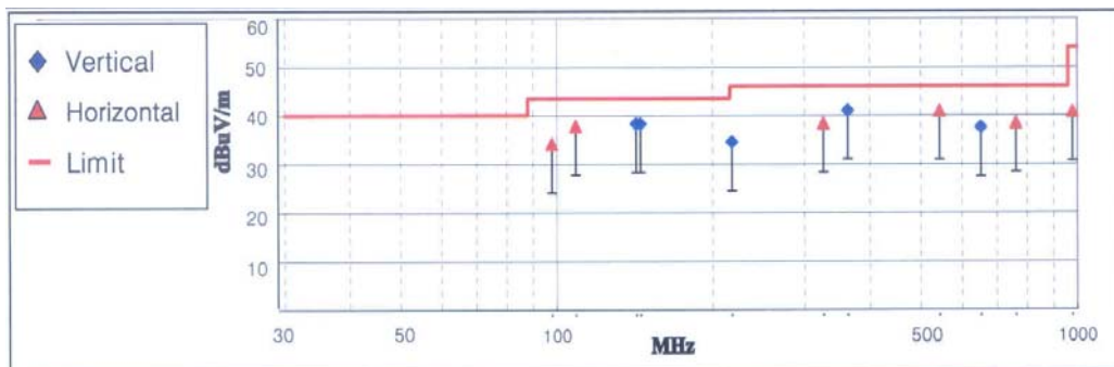
-. Fig 4. Radiated emission result _ Analog
