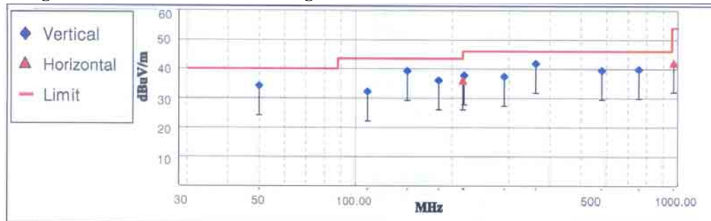
-. Fig 5. Radiated emission result _ Digital
