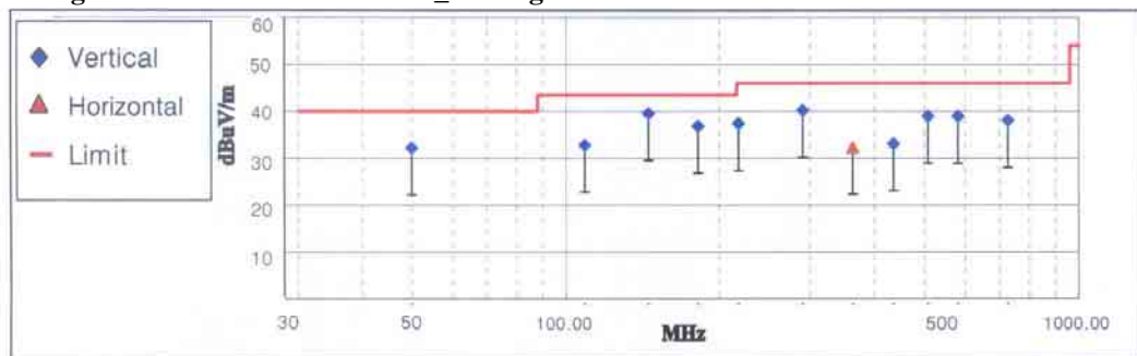
-. Fig 4. Radiated emission result _ Analog
