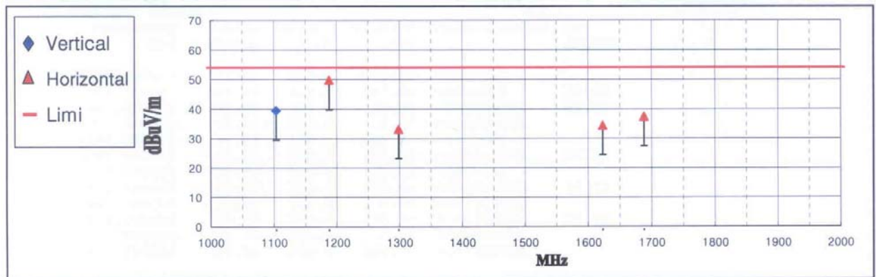
< Fig 5. Radiated emission result _1000M ~ 2000MHz (Analog) >
