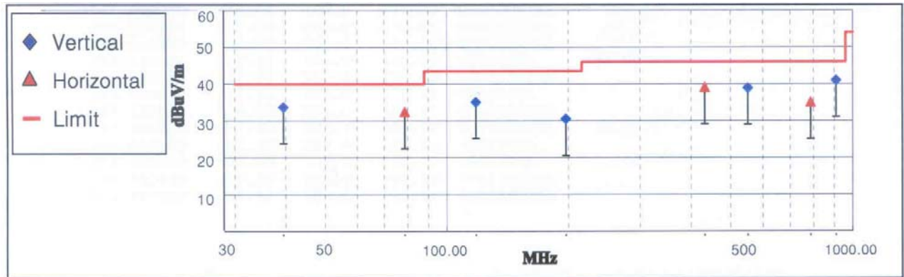
< Fig 4. Radiated emission result _30M ~ 1000MHz (Analog) >
