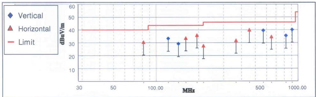
< Fig 6. Radiated emission result _ 30M ~ 1000MHz (Digital) >
