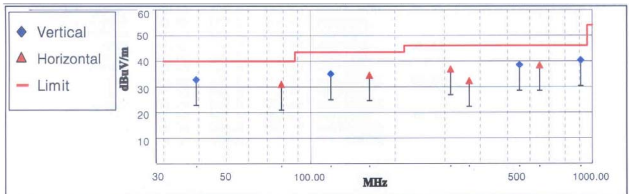
< Fig 8. Radiated emission result >
