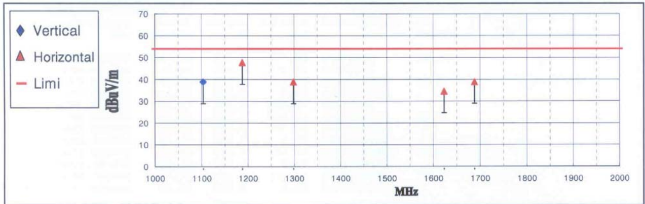
< Fig 7. Radiated emission result _1000M ~ 2000MHz (Digital) >
