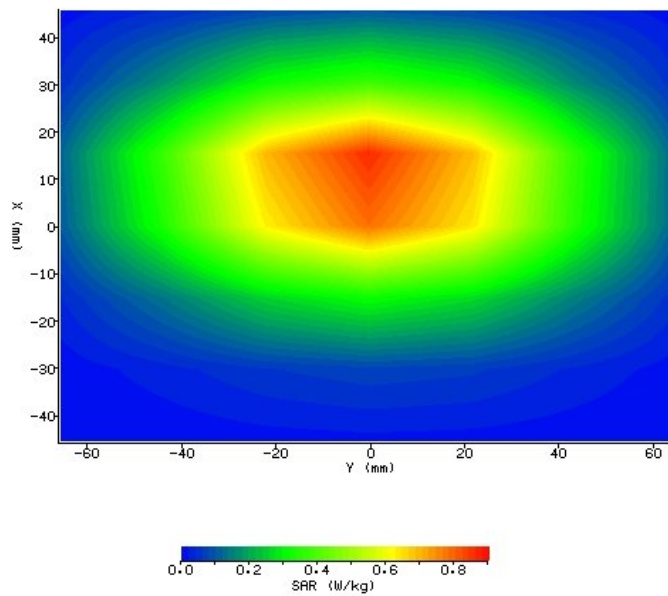
Validation Measurement – 835 MHz in Head tissue
