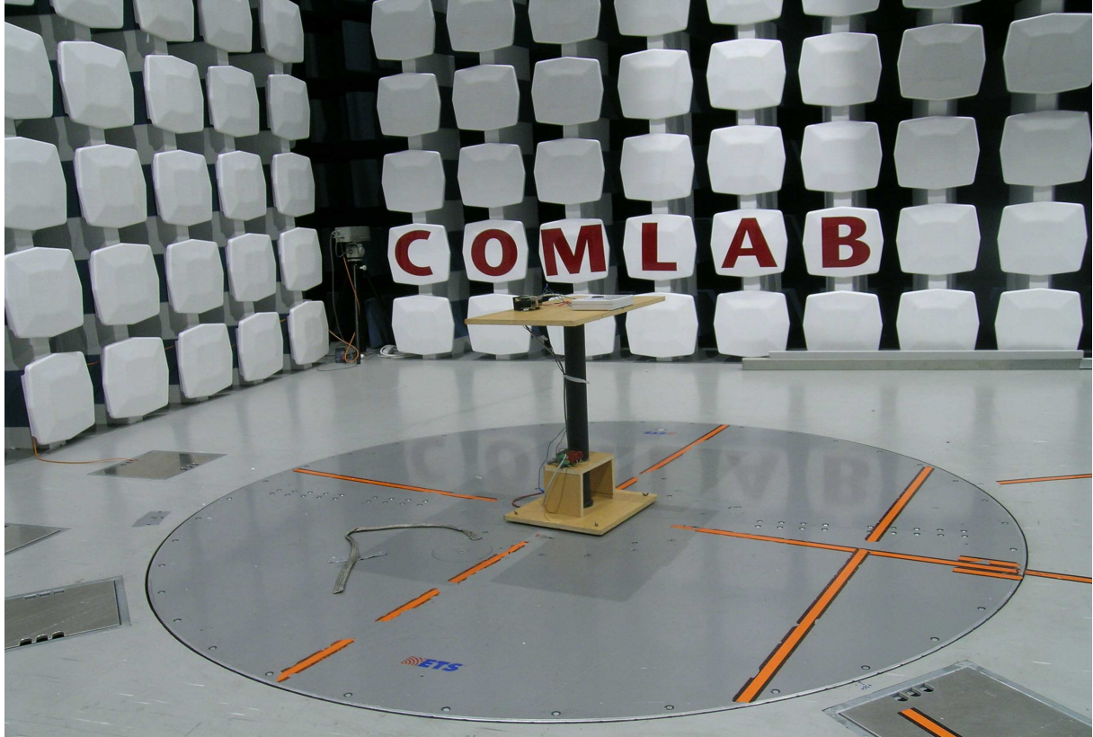
ECU-01- Radiated emission 9 kHz – 10 GHz
