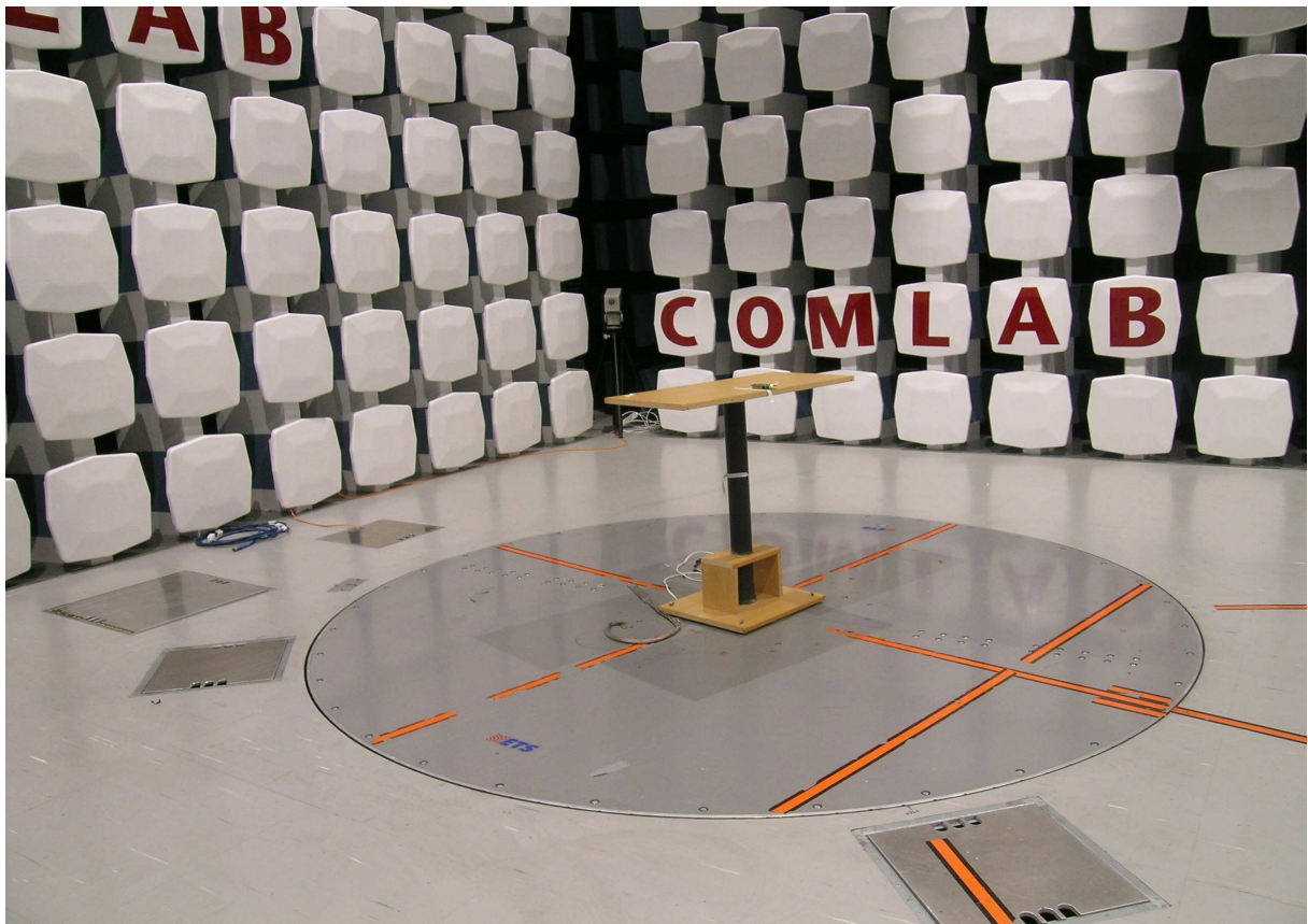
RC-01 – Radiated emission – 9kHz – 10GHz
