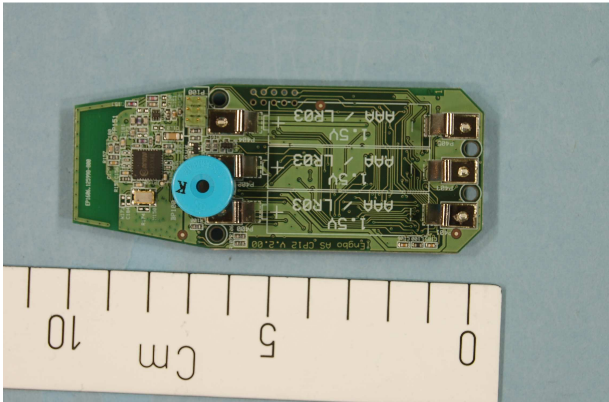
RC-01 – View of PCB – Battery side
