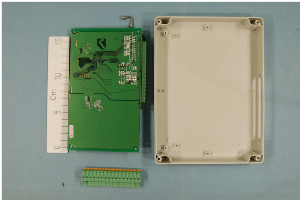
ECU-01 – rear side of the PCB
