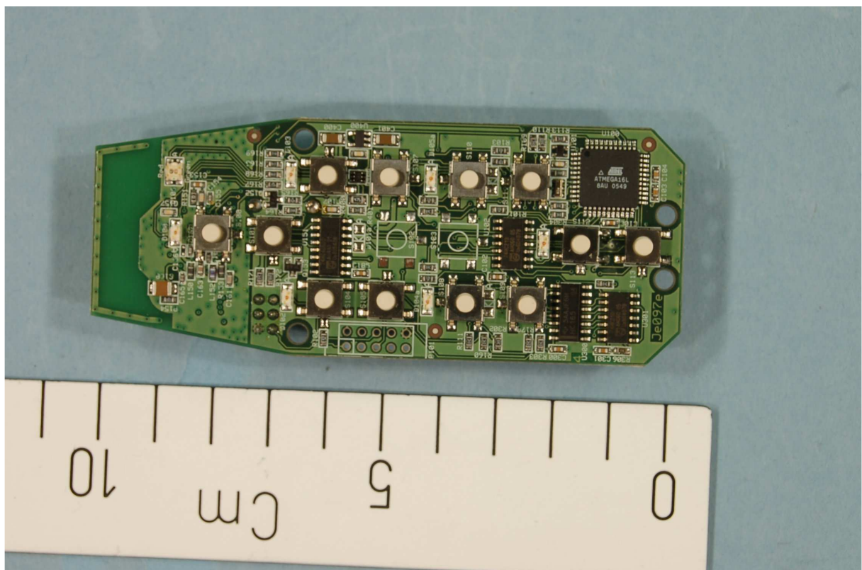
RC-01 – View of PCB – Switch board side
