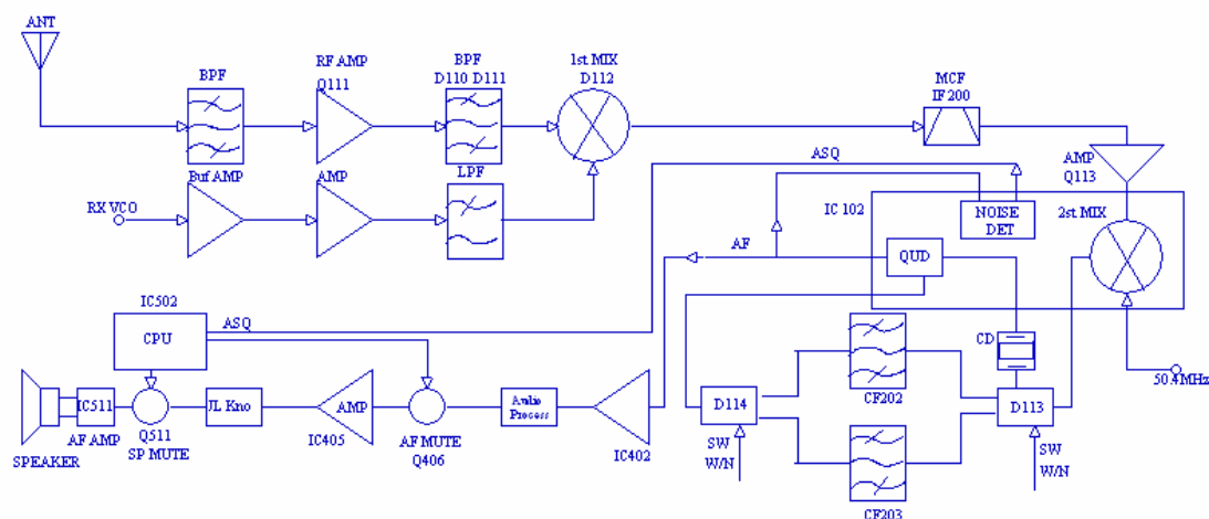
Fig 1 Receiver Circuit
