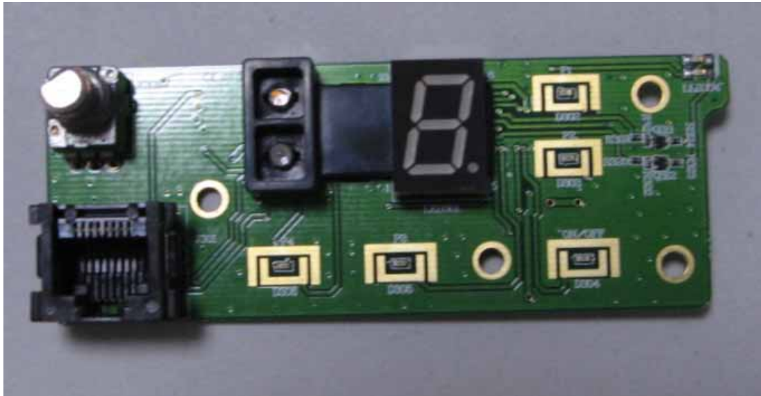
Internal Photo of Front Panel-1
