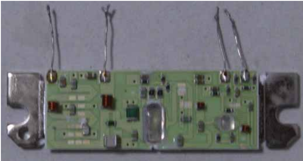
Internal Photo of Radio -1
