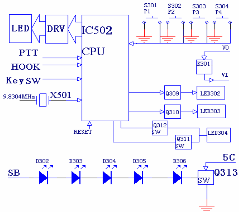
Display Circuit Block Diagram
