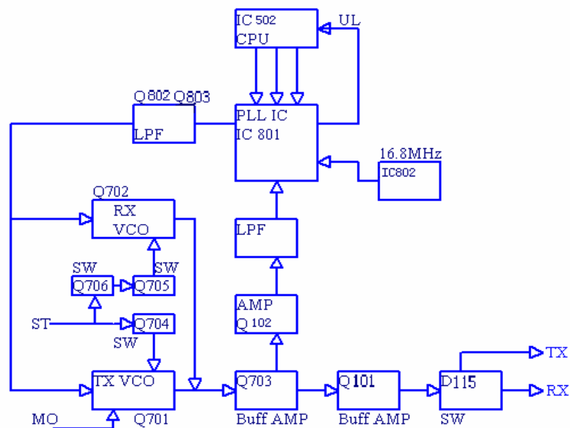
Fig3 PLL Circuit
