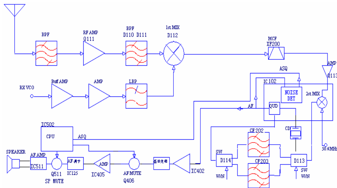
Figure 1 Receiver Section Configuration
