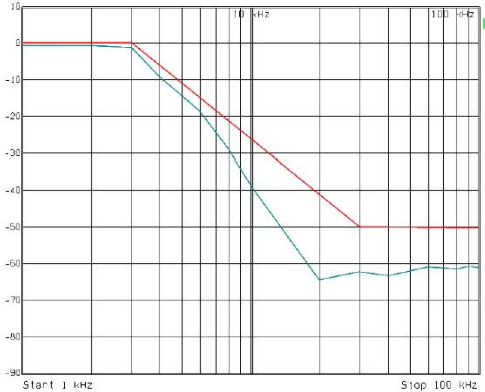
Audio Low Pass Filter Response
