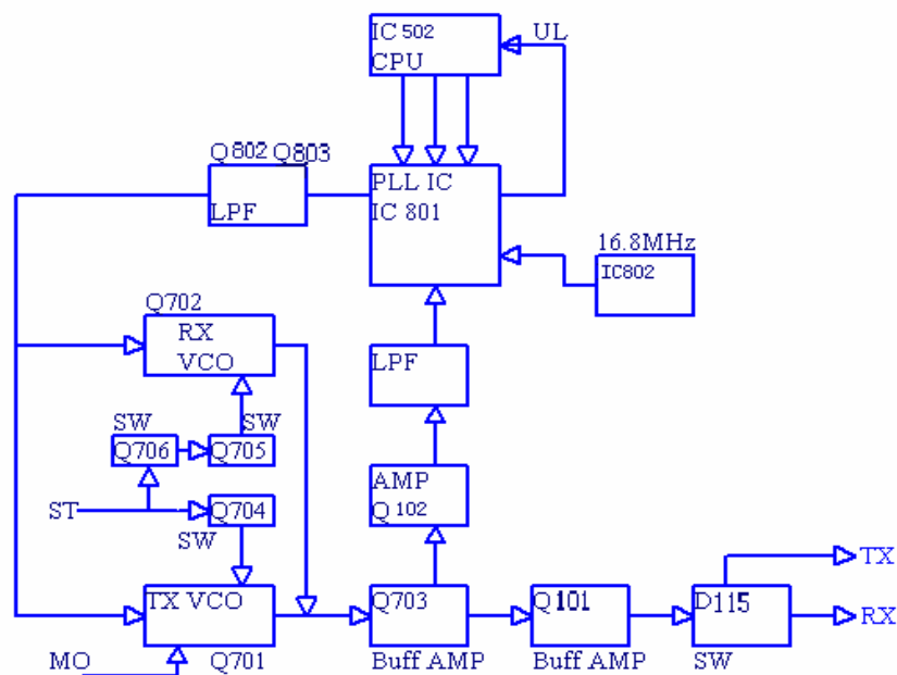
Fig3 PLL Circuit
