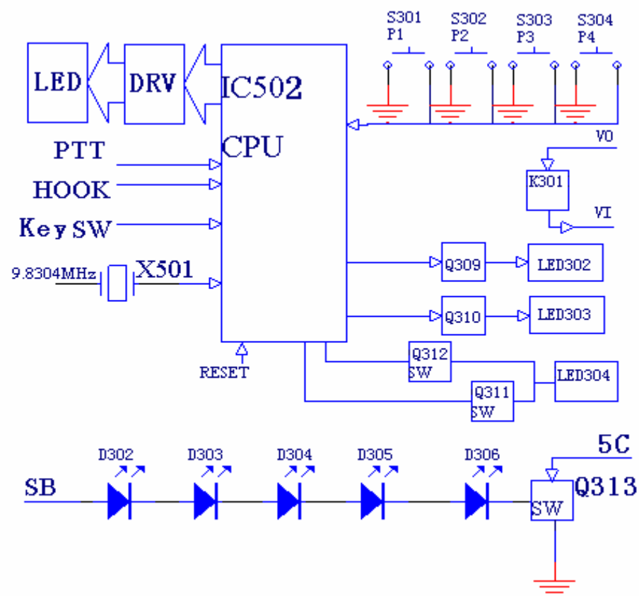
Fig6. Display Circuit
