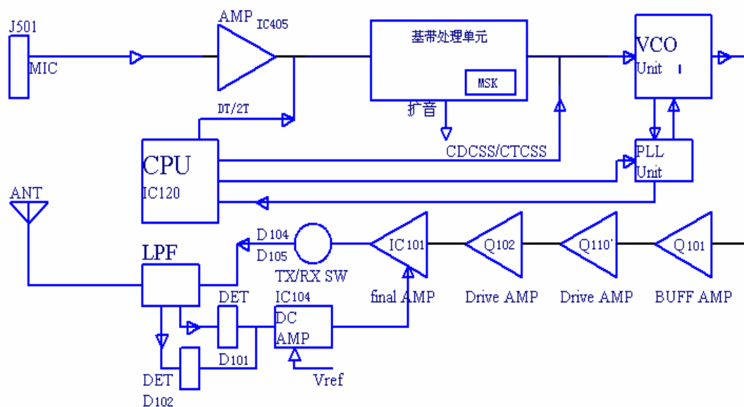
Fig2 Transmitter Circuit
