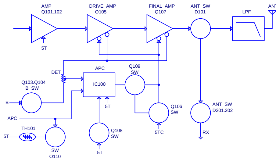
Fig.4 APC System
