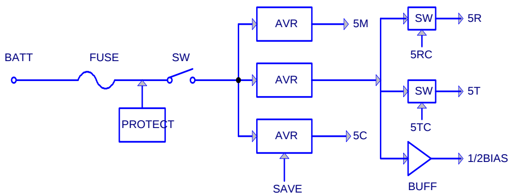
Fig. 1 Power Supply Block Diagram
