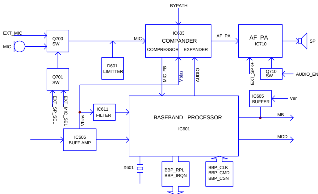
Fig.5 AF and Signalling Circuit
