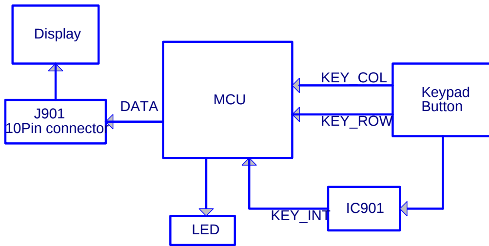
Fig.7 Keypad and Display Block Diagram
