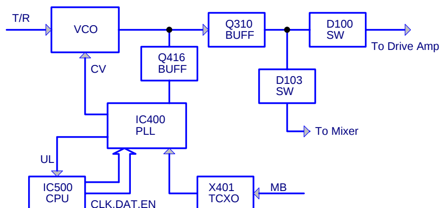
Fig2. PLL circuit
