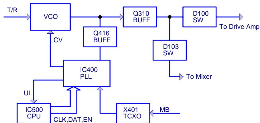
Fig2. PLL circuit
