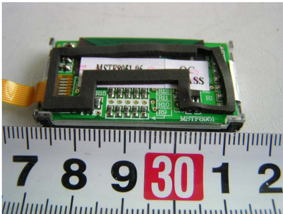
EUT – LCD PCB Rear View
