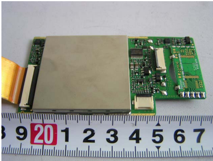
EUT – Keyboard PCB Rear View (1)
