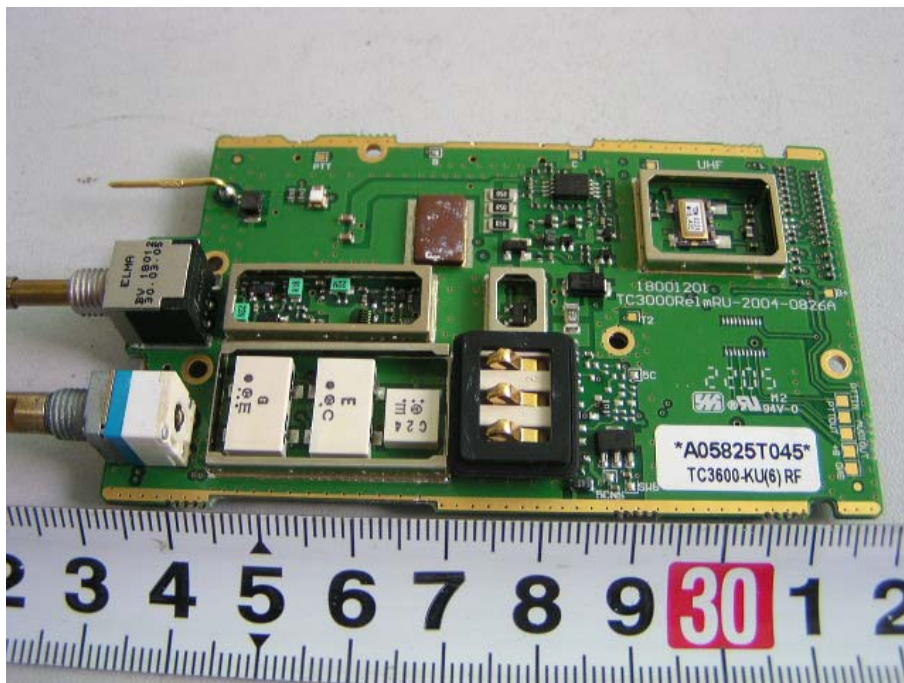
EUT – Main PCB Front View (2)
