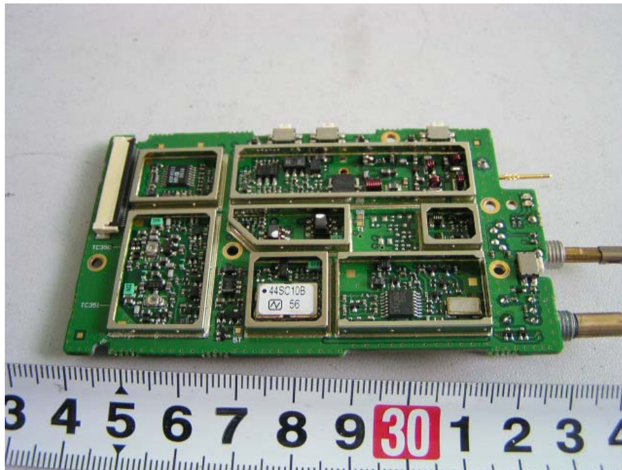
EUT – Main PCB Rear View (2)
