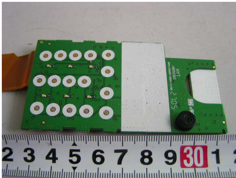
EUT – Keyboard PCB Front View
