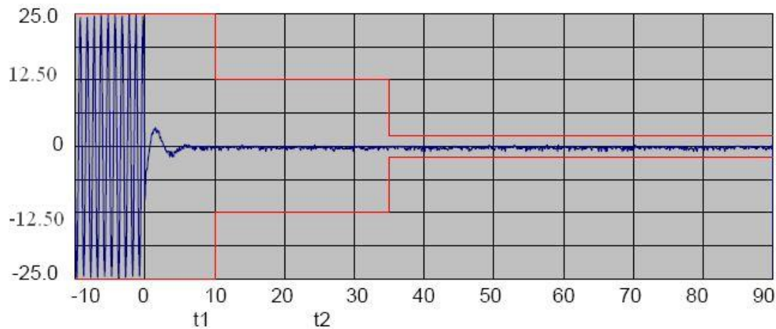
Transmitter Frequency Behaviour @ 25 KHz Channel Separation-----Off – On
