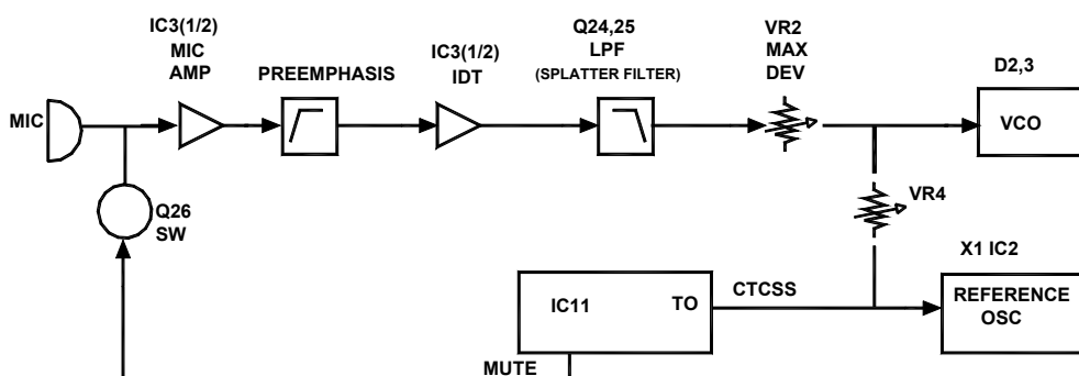
Figure 6. transmit CTCSS
