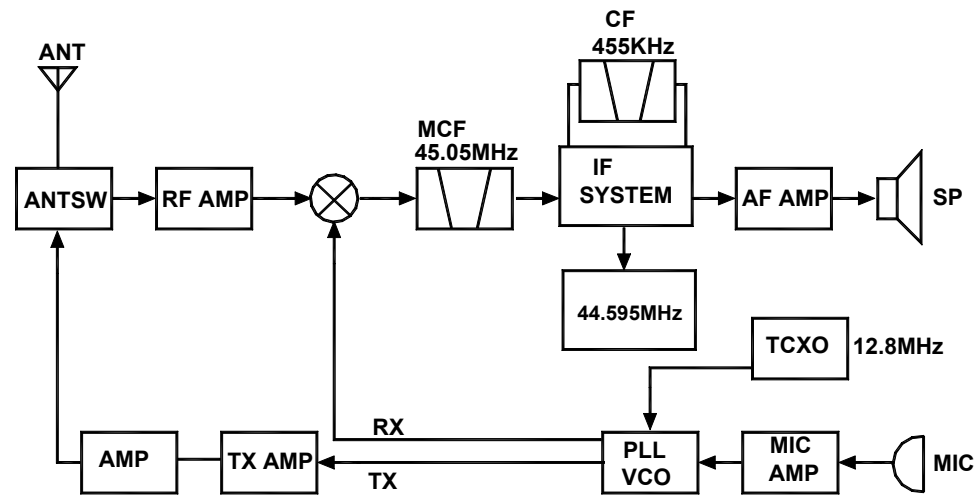
Figure 1. frequency configuration
