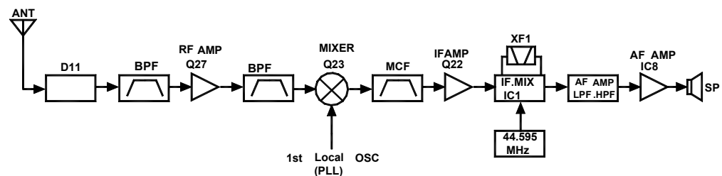
Figure 2. receiver section configuration
