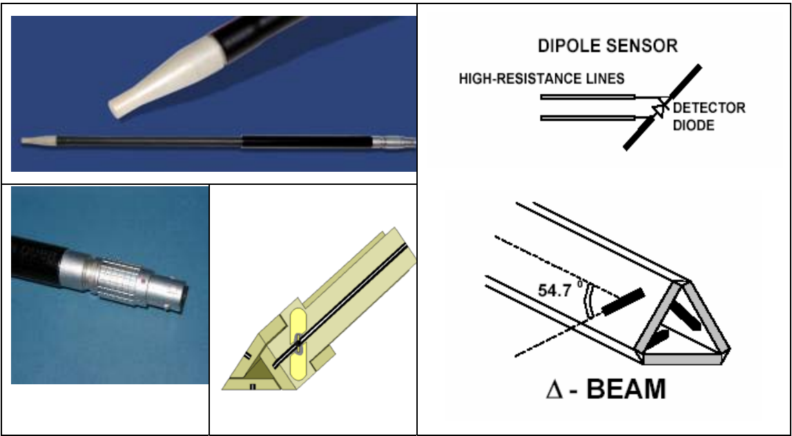
Figure2. Specification and characterization parameters of index sar probe
