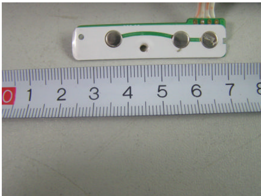
EUT – Key PCB Front View
