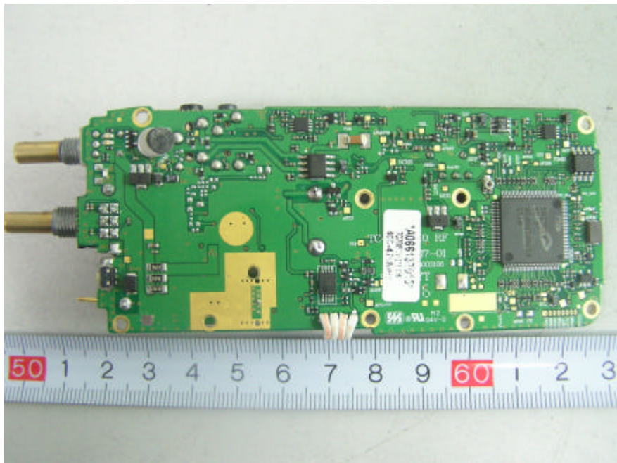
EUT – Main PCB Rear View
