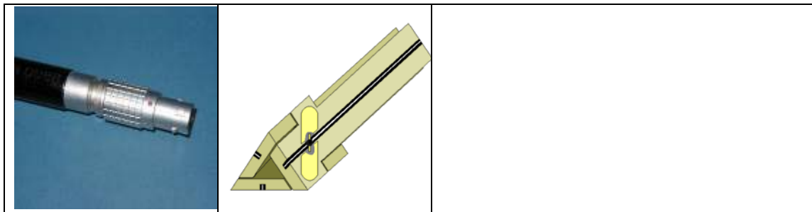
Figure2. Specification and characterization parameters of indexsar probe
