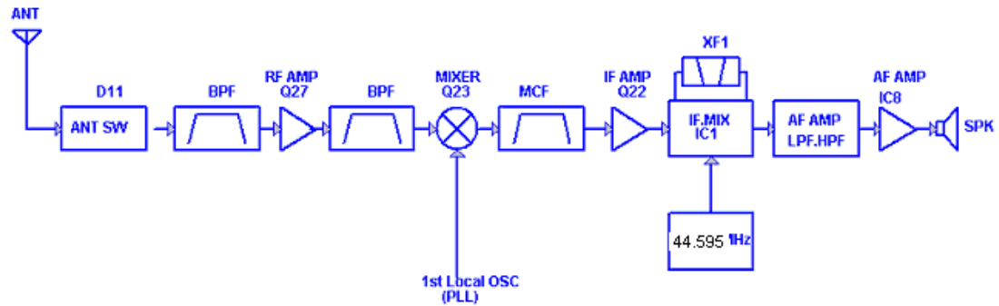
Figure 2 receiver section configuration
