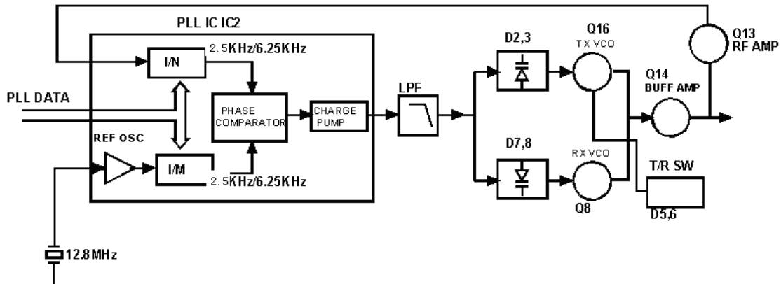
Figure 4 PLL circuit
