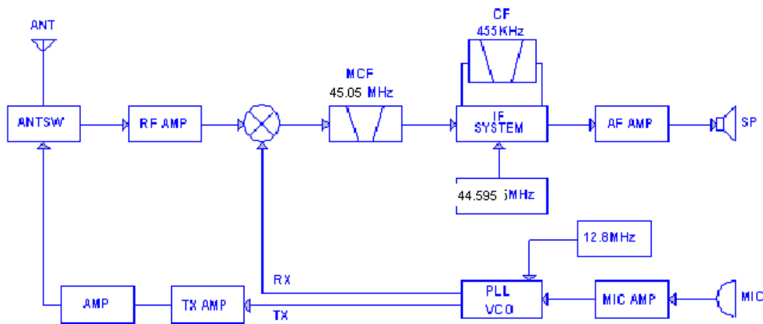
Figure 1 frequency configuration
