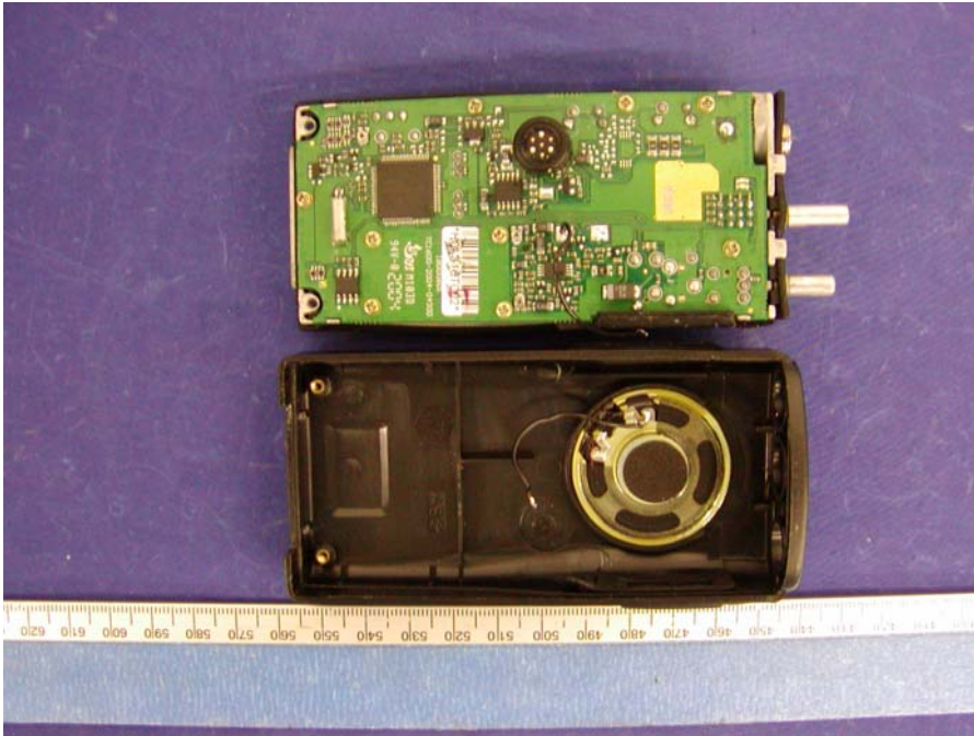
EUT – Board and Housing View
