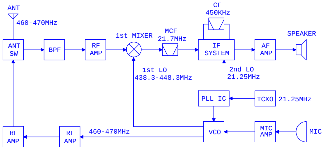
Fig1. Frequency Configuration
