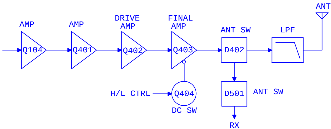
Fig.6 Transmit Module
