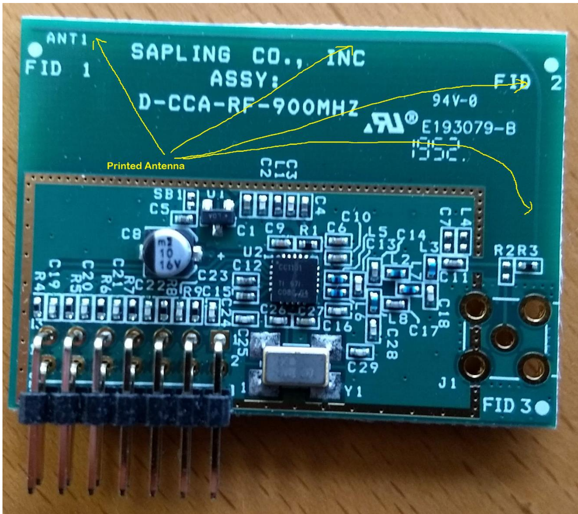
The figure shows the PCB printed antenna:
