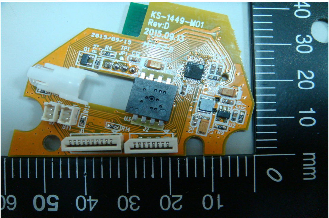
< PCB3-F >
