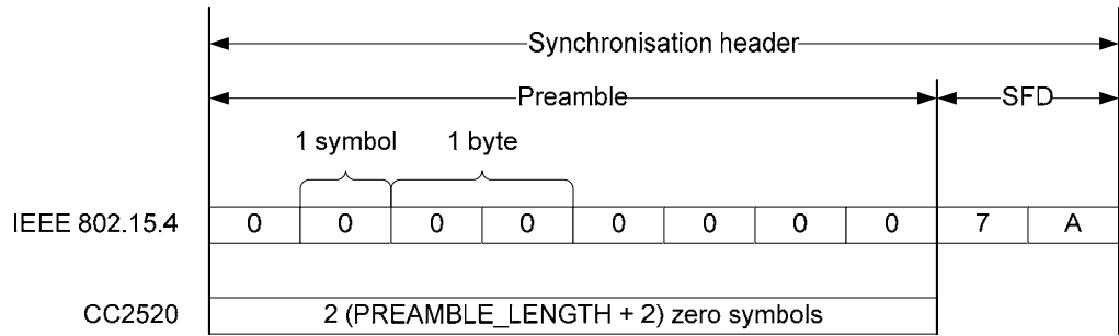
Figure 18: Transmitted Synchronisation Header
