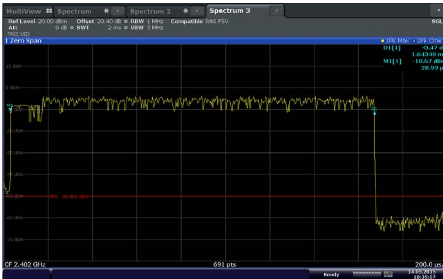
\pi/4 -DQPSK width of single pulse (1.64348 ms)
