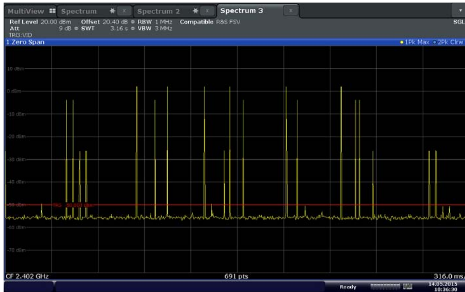
6 pulses/3.16 seconds ( \pi/4 -DQPSK)
