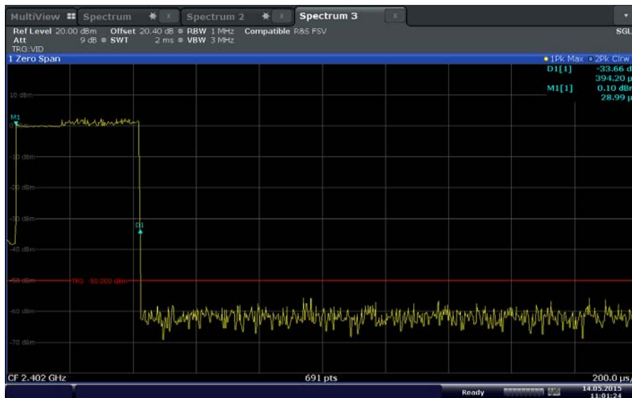
8PSK width of single pulse (0.3942 ms)
