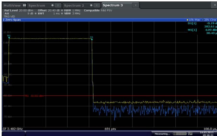
GFSK width of single pulse (0.38261ms)
