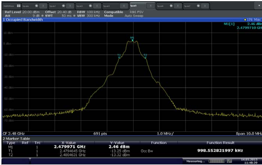
GFSK High Channel
