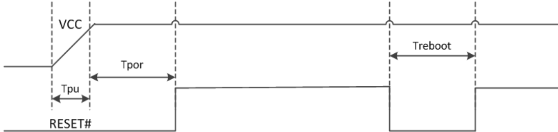
Figure 8-1 Reset Timing
