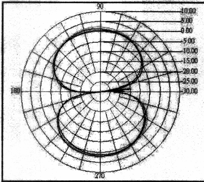
E-plane For 2.4 GHz
