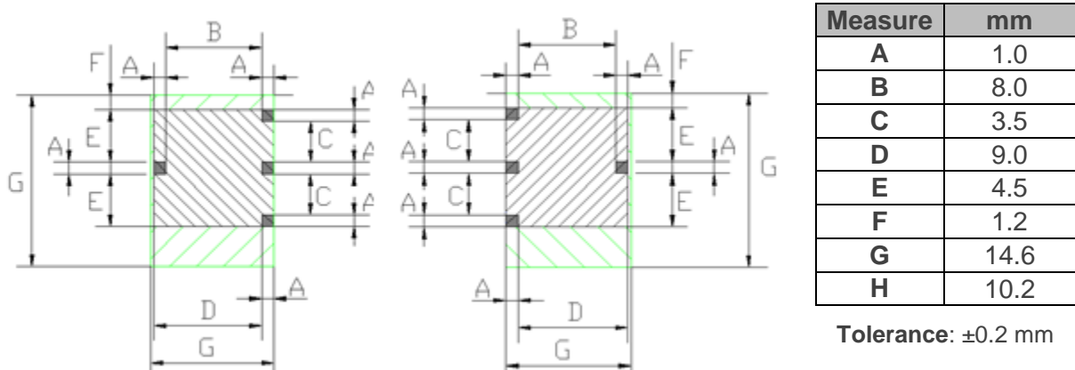
Figure 5 – Antenna Footprint Details
